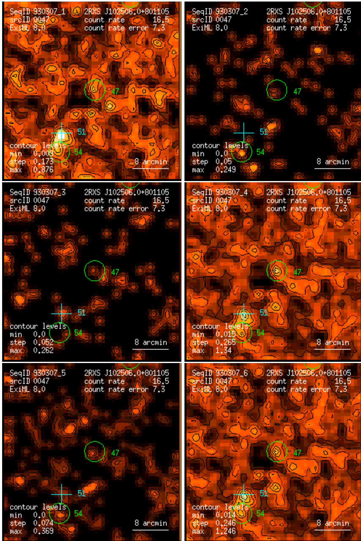
Figure 47: RASS 930307: detection 0047: band rate images, Gaussian filter: (1) PSPC channels 11 – 41, (2) 52 – 90, (3) 91 – 201, (4) 11 – 235, (5) 52 – 201, (6) 11 – 201. Broad band rates in counts/ks. Band rate contour levels in counts/ks/arcmin 2 .
