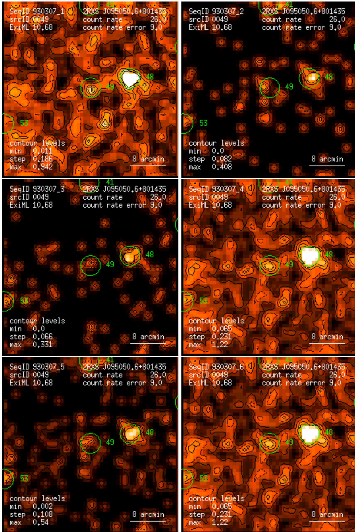
Figure 49: RASS 930307: detection 0049: band rate images, Gaussian filter: (1) PSPC channels 11 – 41, (2) 52 – 90, (3) 91 – 201, (4) 11 – 235, (5) 52 – 201, (6) 11 – 201. Broad band rates in counts/ks. Band rate contour levels in counts/ks/arcmin 2 .
