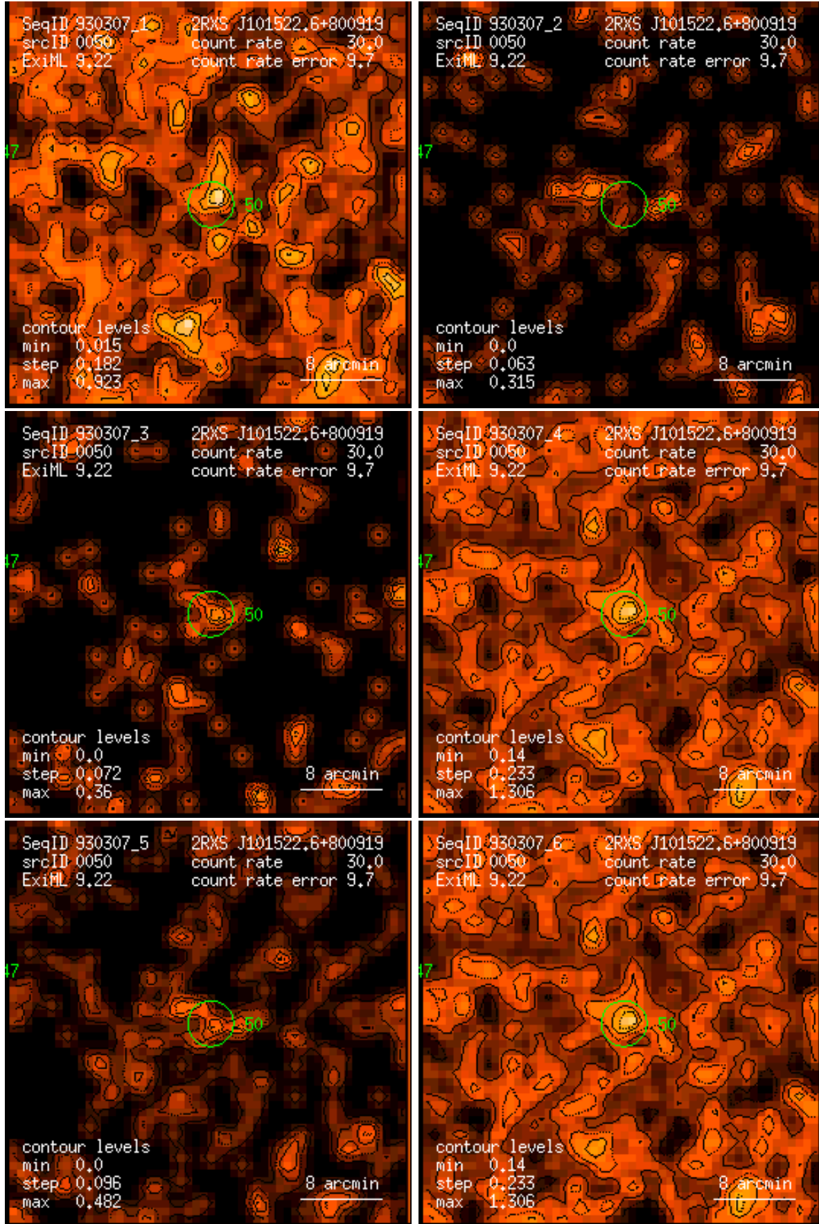
Figure 50: RASS 930307: detection 0050: band rate images, Gaussian filter: (1) PSPC channels 11 – 41, (2) 52 – 90, (3) 91 – 201, (4) 11 – 235, (5) 52 – 201, (6) 11 – 201. Broad band rates in counts/ks. Band rate contour levels in counts/ks/arcmin 2 .
