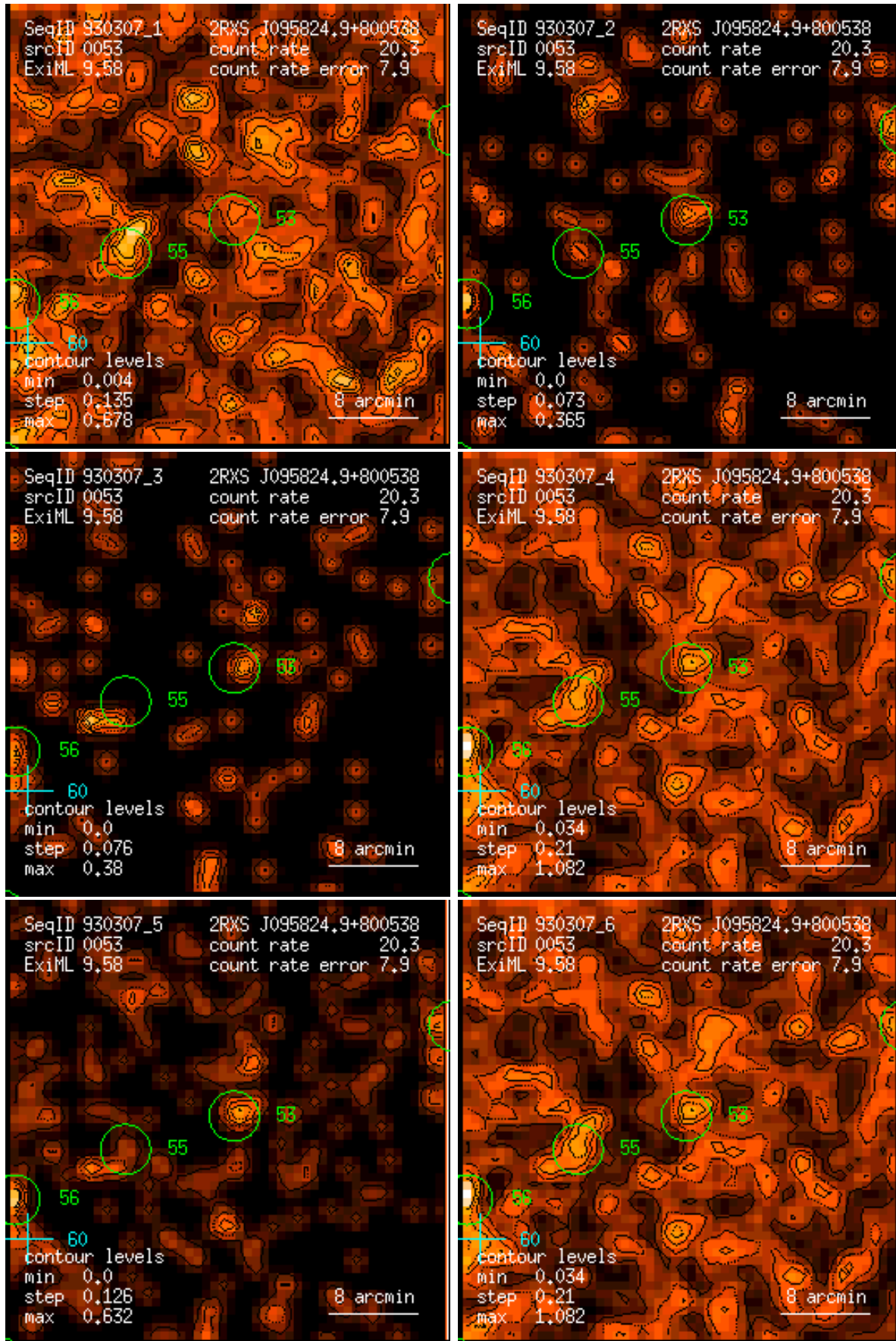
Figure 53: RASS 930307: detection 0053: band rate images, Gaussian filter: (1) PSPC channels 11 – 41, (2) 52 – 90, (3) 91 – 201, (4) 11 – 235, (5) 52 – 201, (6) 11 – 201. Broad band rates in counts/ks. Band rate contour levels in counts/ks/arcmin 2 .
