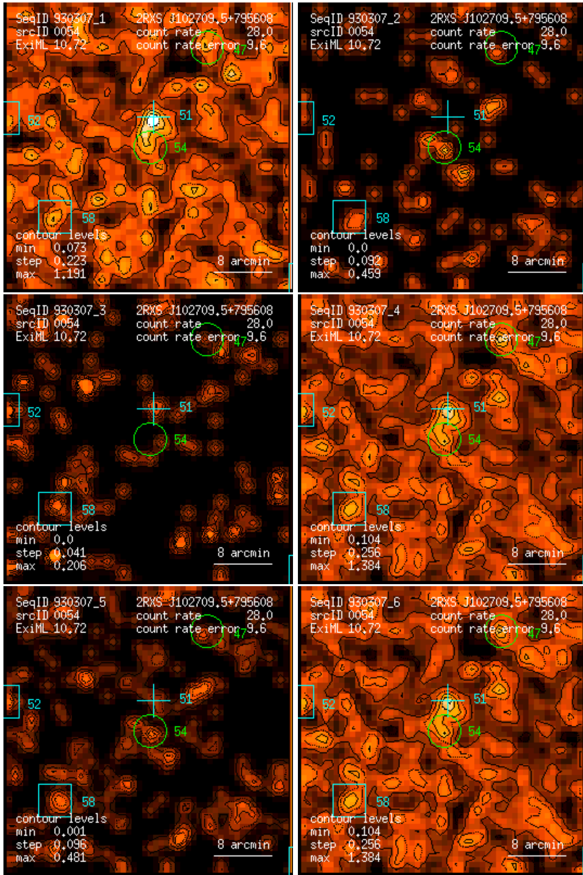
Figure 54: RASS 930307: detection 0054: band rate images, Gaussian filter: (1) PSPC channels 11 – 41, (2) 52 – 90, (3) 91 – 201, (4) 11 – 235, (5) 52 – 201, (6) 11 – 201. Broad band rates in counts/ks. Band rate contour levels in counts/ks/arcmin 2 .
