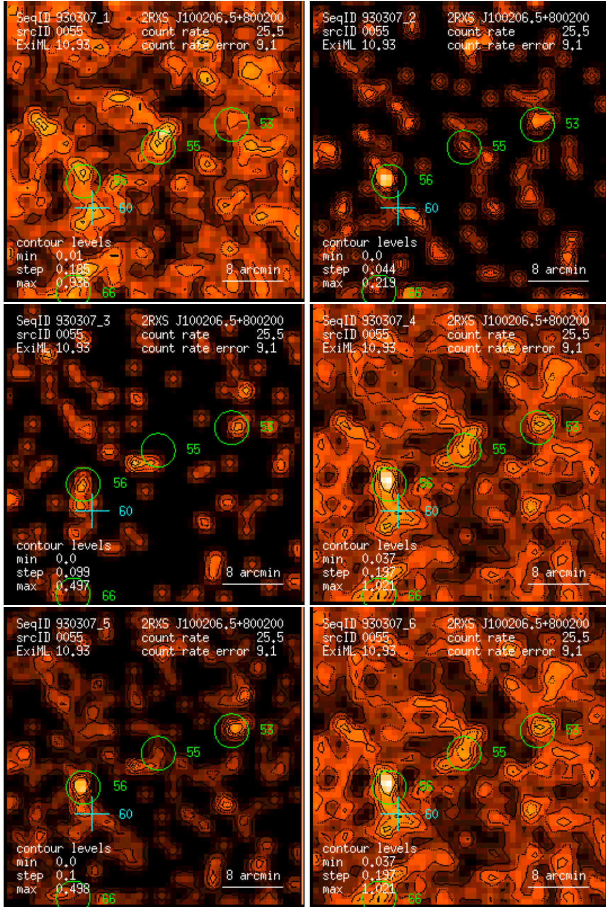
Figure 55: RASS 930307: detection 0055: band rate images, Gaussian filter: (1) PSPC channels 11 – 41, (2) 52 – 90, (3) 91 – 201, (4) 11 – 235, (5) 52 – 201, (6) 11 – 201. Broad band rates in counts/ks. Band rate contour levels in counts/ks/arcmin 2 .
