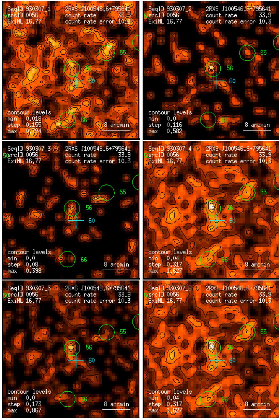
Figure 56: RASS 930307: detection 0056: band rate images, Gaussian filter: (1) PSPC channels 11 – 41, (2) 52 – 90, (3) 91 – 201, (4) 11 – 235, (5) 52 – 201, (6) 11 – 201. Broad band rates in counts/ks. Band rate contour levels in counts/ks/arcmin 2 .
