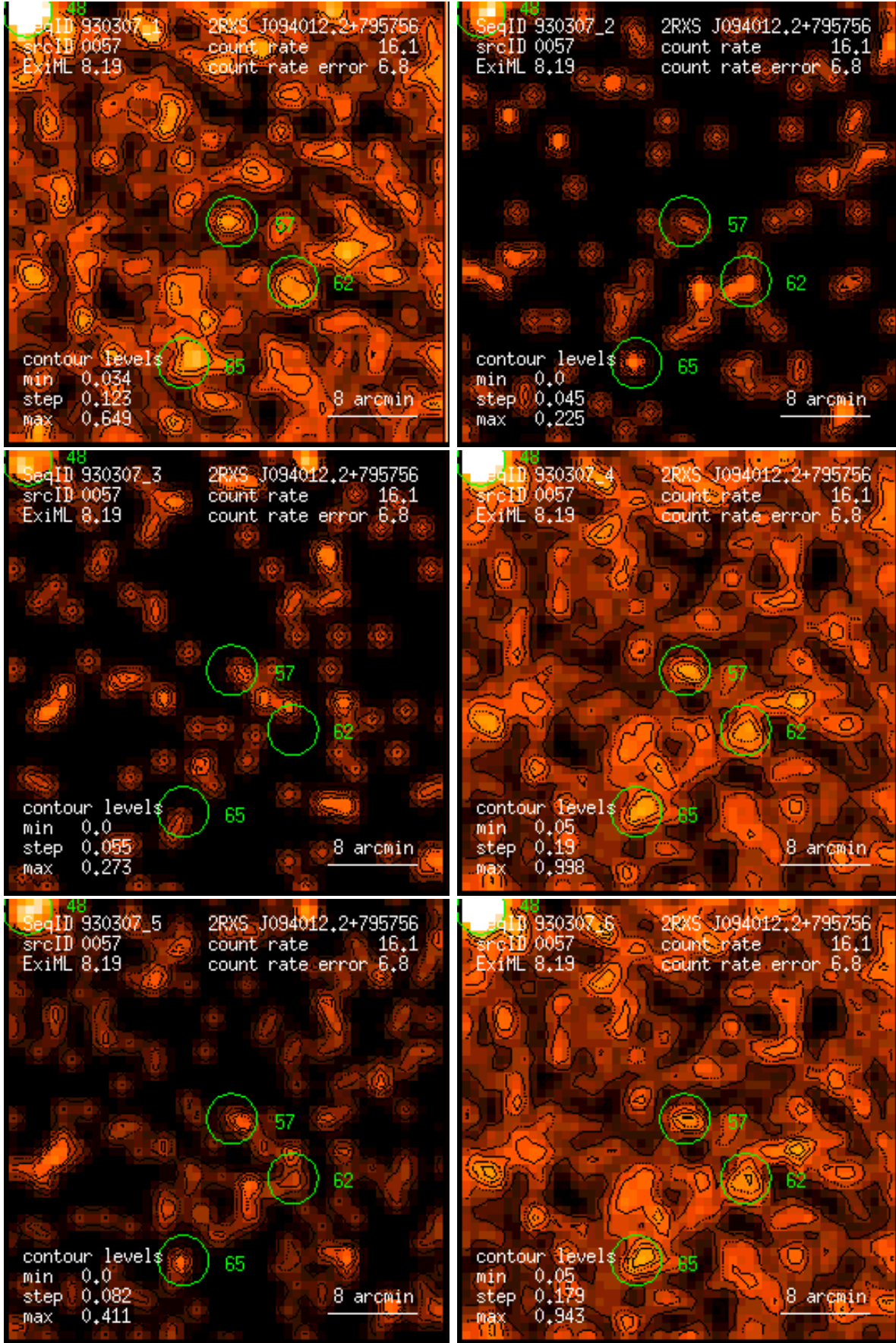
Figure 57: RASS 930307: detection 0057: band rate images, Gaussian filter: (1) PSPC channels 11 – 41, (2) 52 – 90, (3) 91 – 201, (4) 11 – 235, (5) 52 – 201, (6) 11 – 201. Broad band rates in counts/ks. Band rate contour levels in counts/ks/arcmin 2 .
