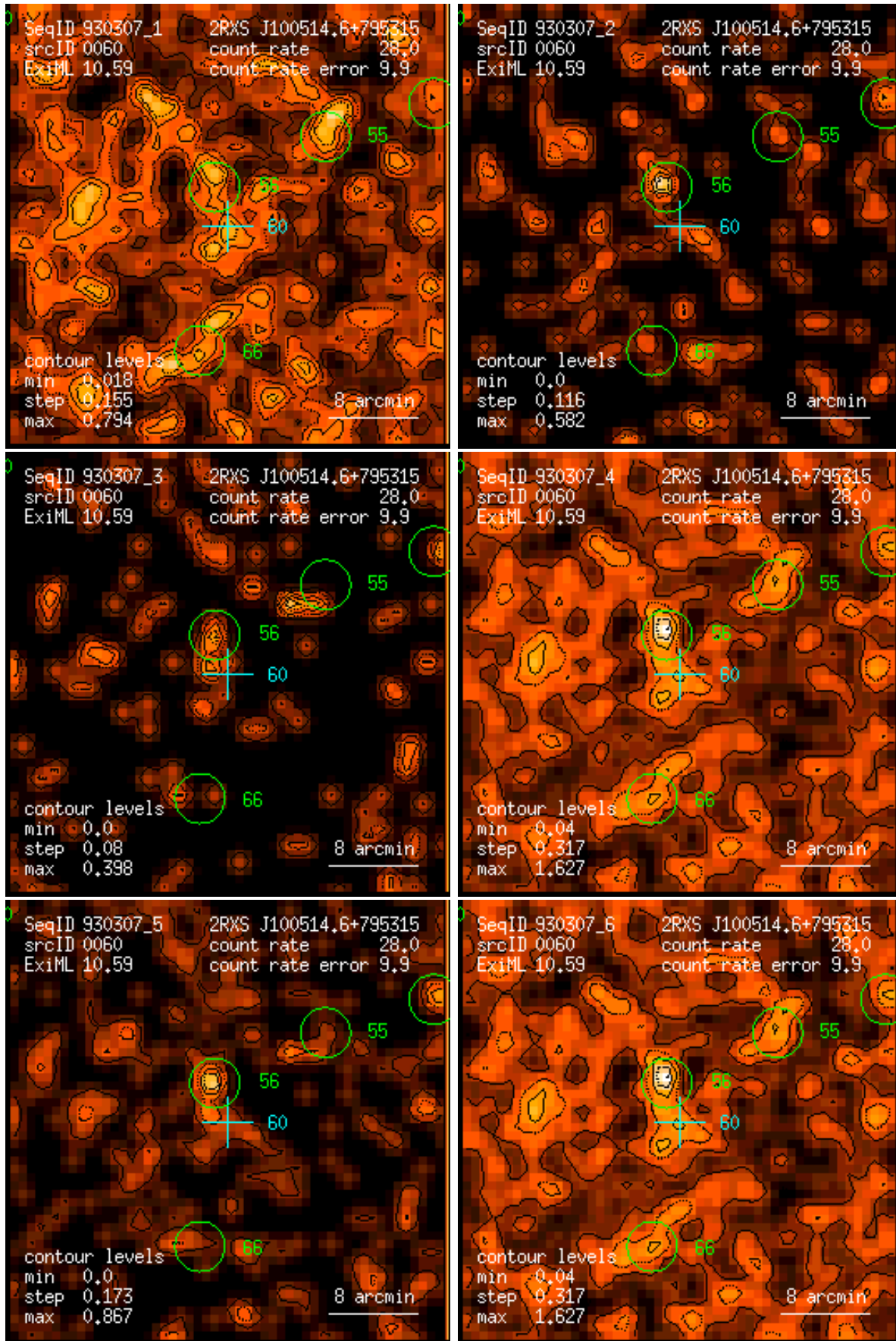
Figure 60: RASS 930307: detection 0060: band rate images, Gaussian filter: (1) PSPC channels 11 – 41, (2) 52 – 90, (3) 91 – 201, (4) 11 – 235, (5) 52 – 201, (6) 11 – 201. Broad band rates in counts/ks. Band rate contour levels in counts/ks/arcmin 2 .
