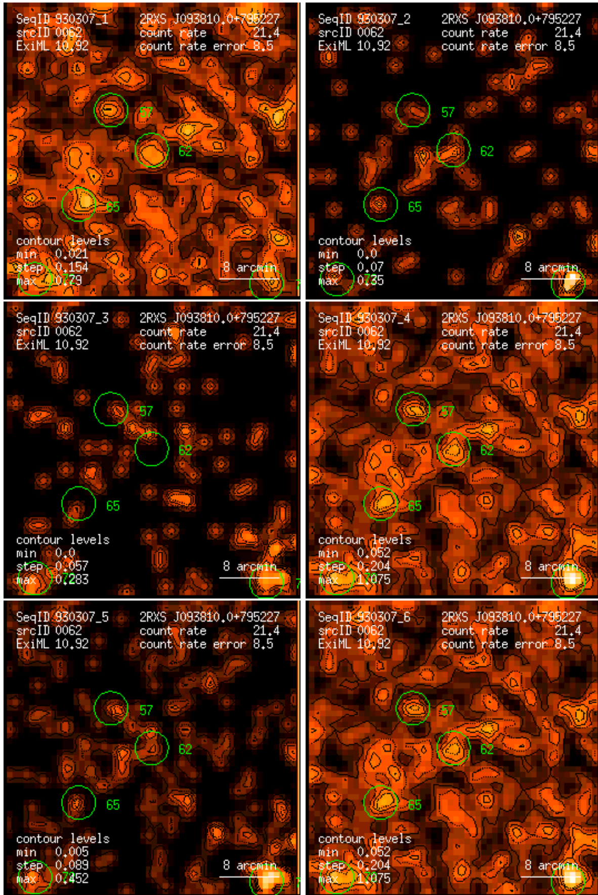
Figure 62: RASS 930307: detection 0062: band rate images, Gaussian filter: (1) PSPC channels 11 – 41, (2) 52 – 90, (3) 91 – 201, (4) 11 – 235, (5) 52 – 201, (6) 11 – 201. Broad band rates in counts/ks. Band rate contour levels in counts/ks/arcmin 2 .
