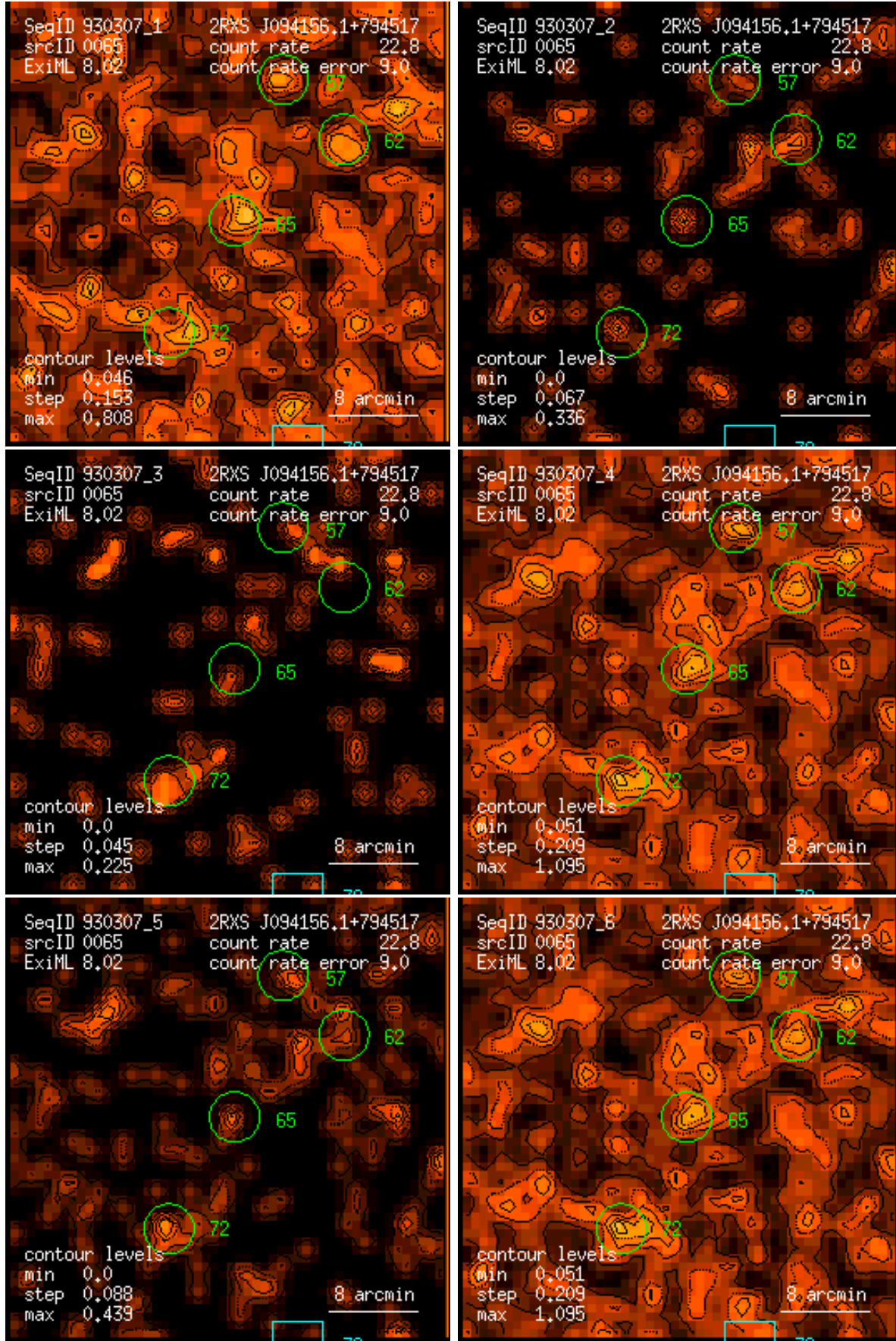
Figure 65: RASS 930307: detection 0065: band rate images, Gaussian filter: (1) PSPC channels 11 – 41, (2) 52 – 90, (3) 91 – 201, (4) 11 – 235, (5) 52 – 201, (6) 11 – 201. Broad band rates in counts/ks. Band rate contour levels in counts/ks/arcmin 2 .
