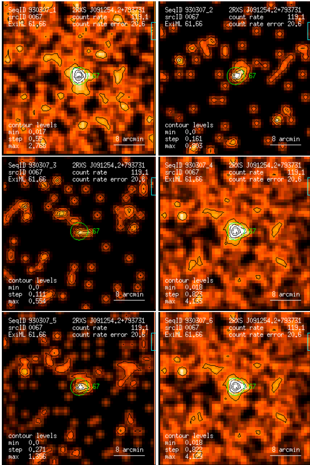
Figure 67: RASS 930307: detection 0067: band rate images, Gaussian filter: (1) PSPC channels 11 – 41, (2) 52 – 90, (3) 91 – 201, (4) 11 – 235, (5) 52 – 201, (6) 11 – 201. Broad band rates in counts/ks. Band rate contour levels in counts/ks/arcmin 2 .
