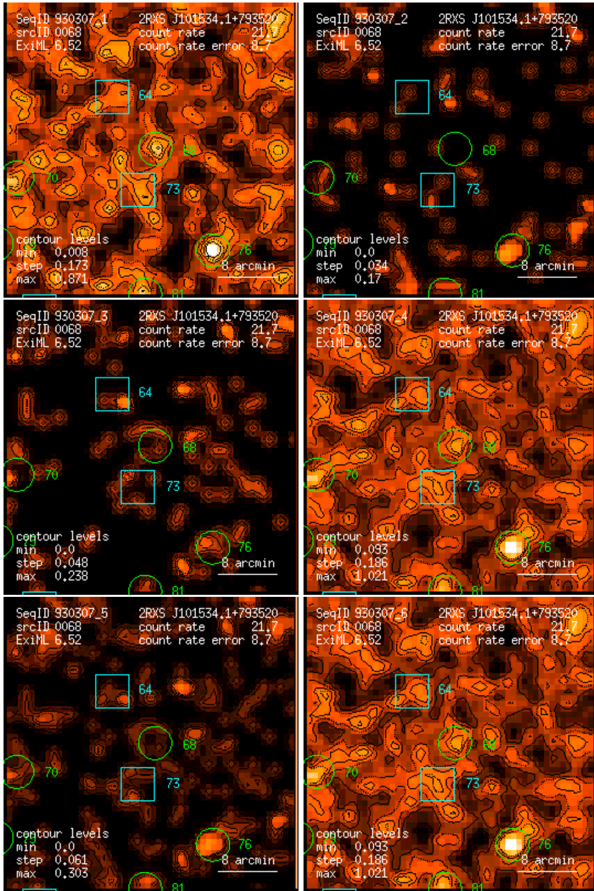
Figure 68: RASS 930307: detection 0068: band rate images, Gaussian filter: (1) PSPC channels 11 – 41, (2) 52 – 90, (3) 91 – 201, (4) 11 – 235, (5) 52 – 201, (6) 11 – 201. Broad band rates in counts/ks. Band rate contour levels in counts/ks/arcmin 2 .
