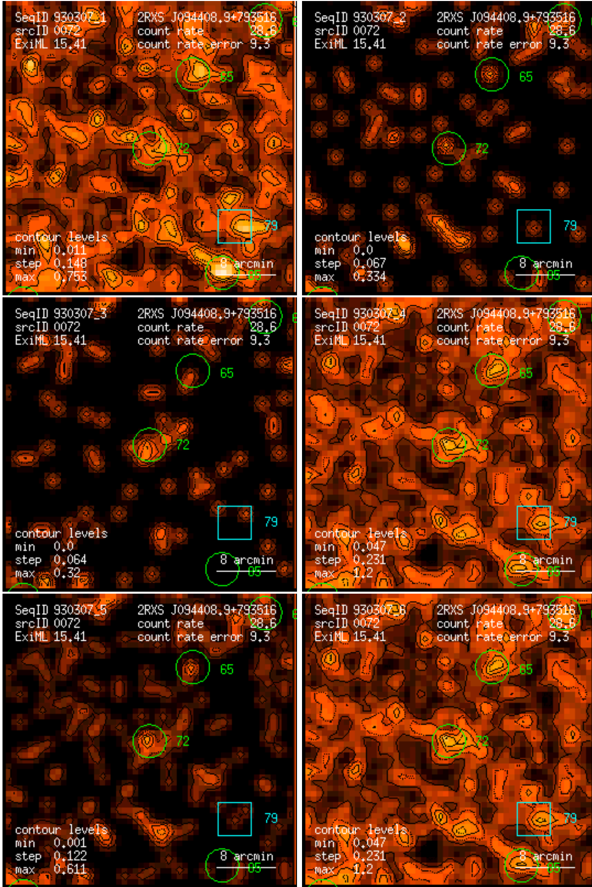
Figure 72: RASS 930307: detection 0072: band rate images, Gaussian filter: (1) PSPC channels 11 – 41, (2) 52 – 90, (3) 91 – 201, (4) 11 – 235, (5) 52 – 201, (6) 11 – 201. Broad band rates in counts/ks. Band rate contour levels in counts/ks/arcmin 2 .
