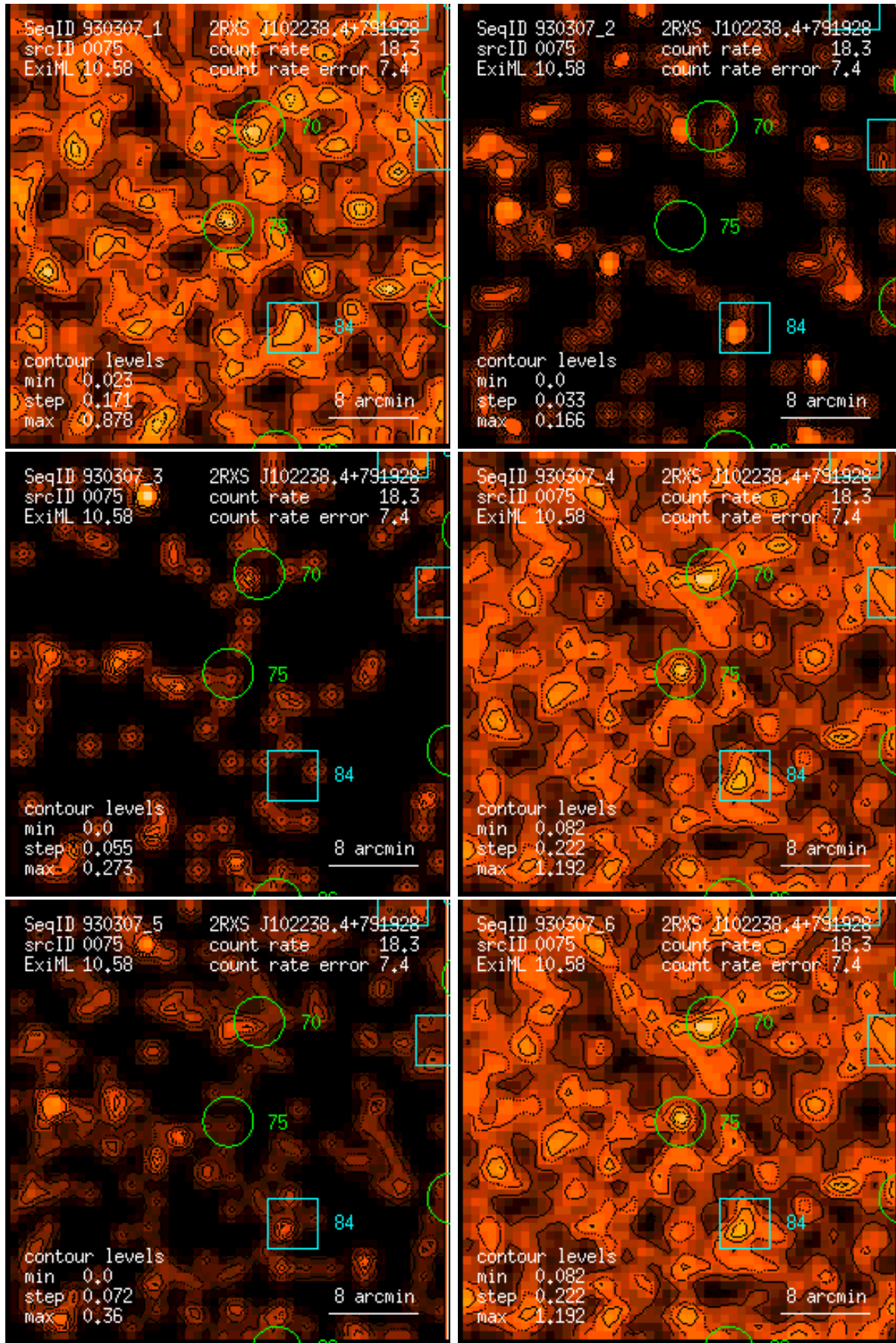
Figure 75: RASS 930307: detection 0075: band rate images, Gaussian filter: (1) PSPC channels 11 – 41, (2) 52 – 90, (3) 91 – 201, (4) 11 – 235, (5) 52 – 201, (6) 11 – 201. Broad band rates in counts/ks. Band rate contour levels in counts/ks/arcmin 2 .
