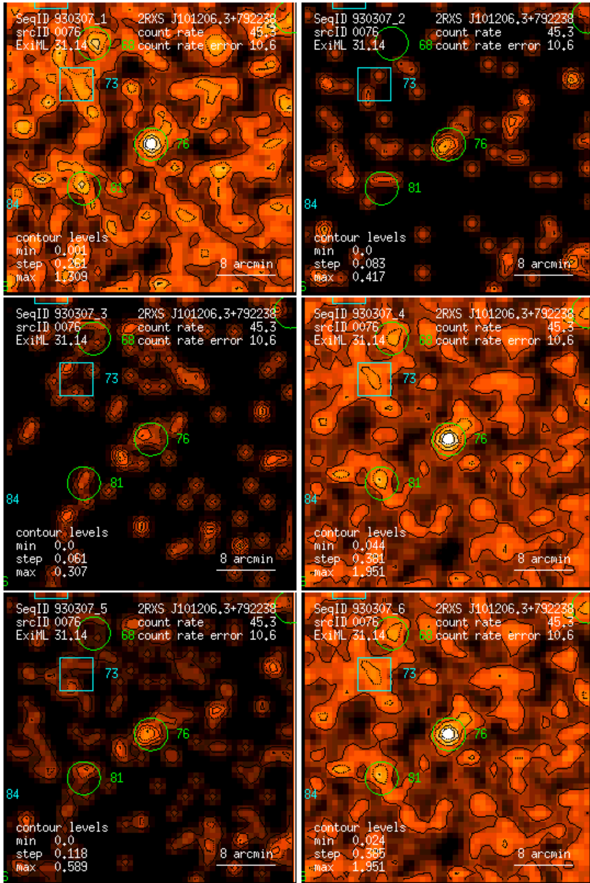
Figure 76: RASS 930307: detection 0076: band rate images, Gaussian filter: (1) PSPC channels 11 – 41, (2) 52 – 90, (3) 91 – 201, (4) 11 – 235, (5) 52 – 201, (6) 11 – 201. Broad band rates in counts/ks. Band rate contour levels in counts/ks/arcmin 2 .
