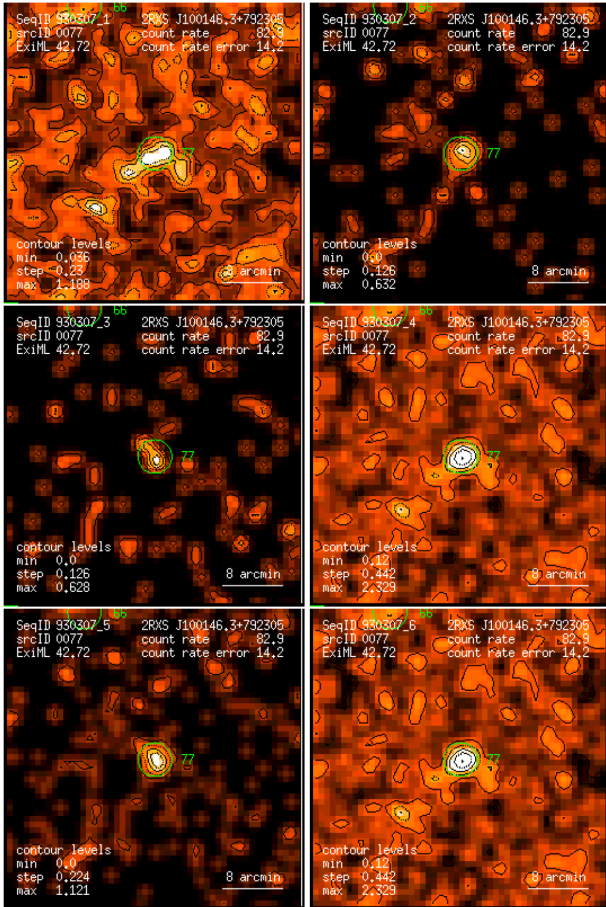
Figure 77: RASS 930307: detection 0077: band rate images, Gaussian filter: (1) PSPC channels 11 – 41, (2) 52 – 90, (3) 91 – 201, (4) 11 – 235, (5) 52 – 201, (6) 11 – 201. Broad band rates in counts/ks. Band rate contour levels in counts/ks/arcmin 2 .
