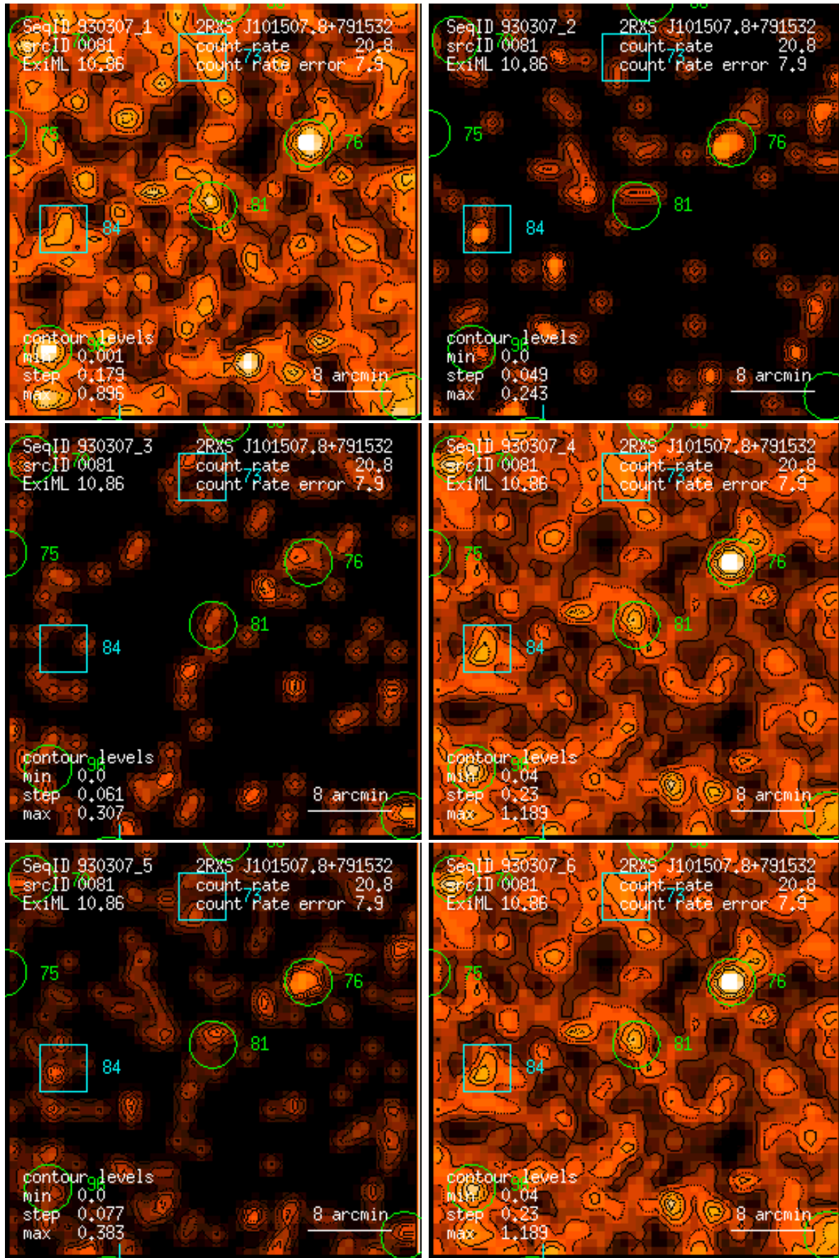
Figure 81: RASS 930307: detection 0081: band rate images, Gaussian filter: (1) PSPC channels 11 – 41, (2) 52 – 90, (3) 91 – 201, (4) 11 – 235, (5) 52 – 201, (6) 11 – 201. Broad band rates in counts/ks. Band rate contour levels in counts/ks/arcmin 2 .
