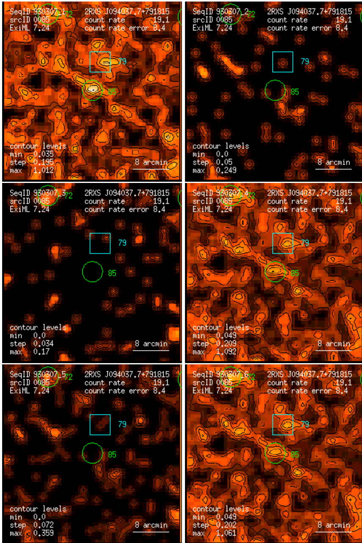
Figure 85: RASS 930307: detection 0085: band rate images, Gaussian filter: (1) PSPC channels 11 – 41, (2) 52 – 90, (3) 91 – 201, (4) 11 – 235, (5) 52 – 201, (6) 11 – 201. Broad band rates in counts/ks. Band rate contour levels in counts/ks/arcmin 2 .
