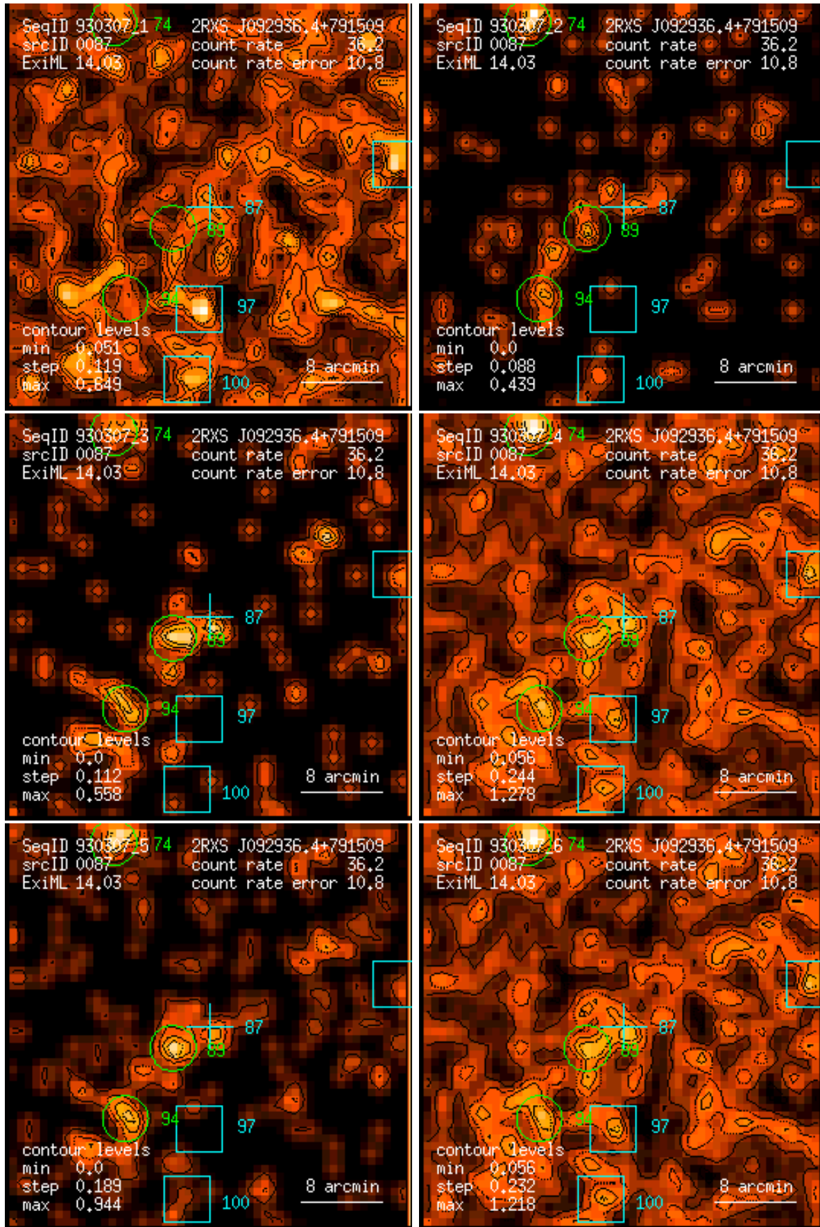
Figure 87: RASS 930307: detection 0087: band rate images, Gaussian filter: (1) PSPC channels 11 – 41, (2) 52 – 90, (3) 91 – 201, (4) 11 – 235, (5) 52 – 201, (6) 11 – 201. Broad band rates in counts/ks. Band rate contour levels in counts/ks/arcmin 2 .
