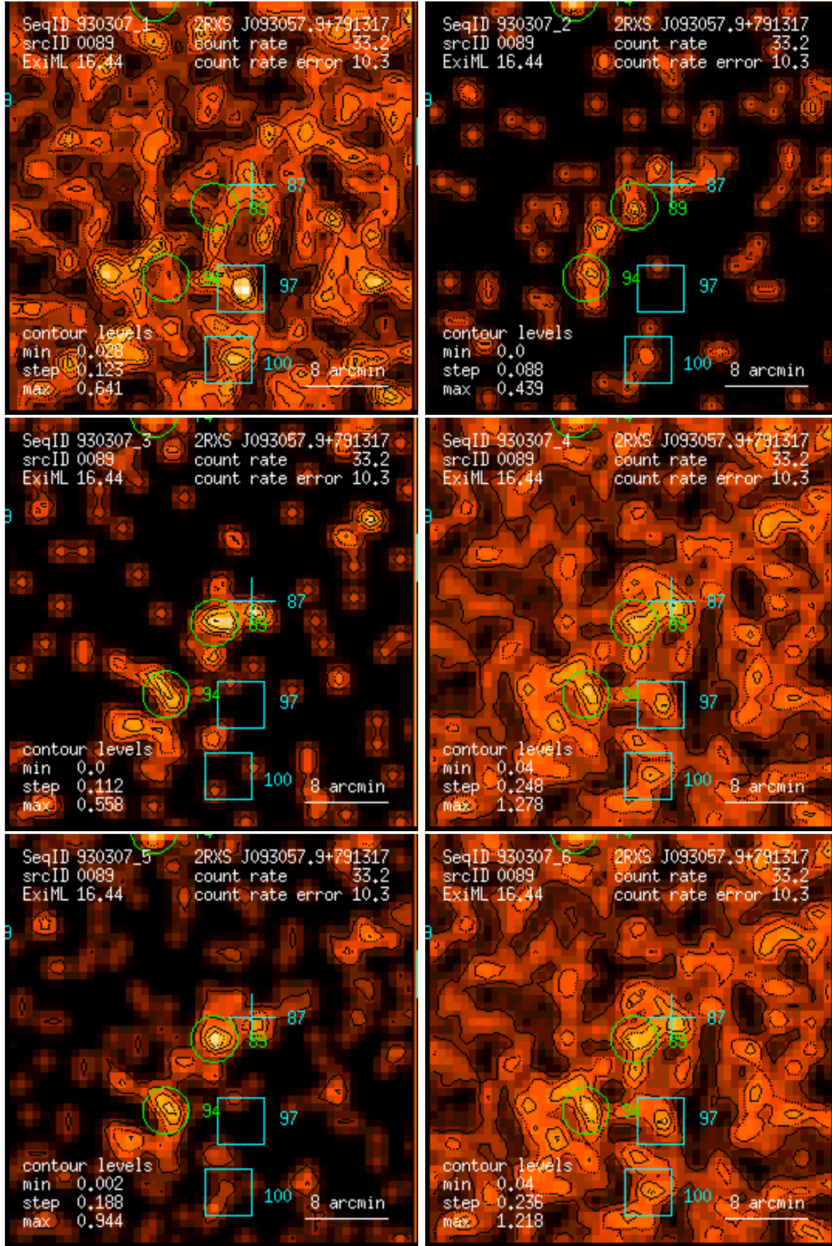
Figure 89: RASS 930307: detection 0089: band rate images, Gaussian filter: (1) PSPC channels 11 – 41, (2) 52 – 90, (3) 91 – 201, (4) 11 – 235, (5) 52 – 201, (6) 11 – 201. Broad band rates in counts/ks. Band rate contour levels in counts/ks/arcmin 2 .
