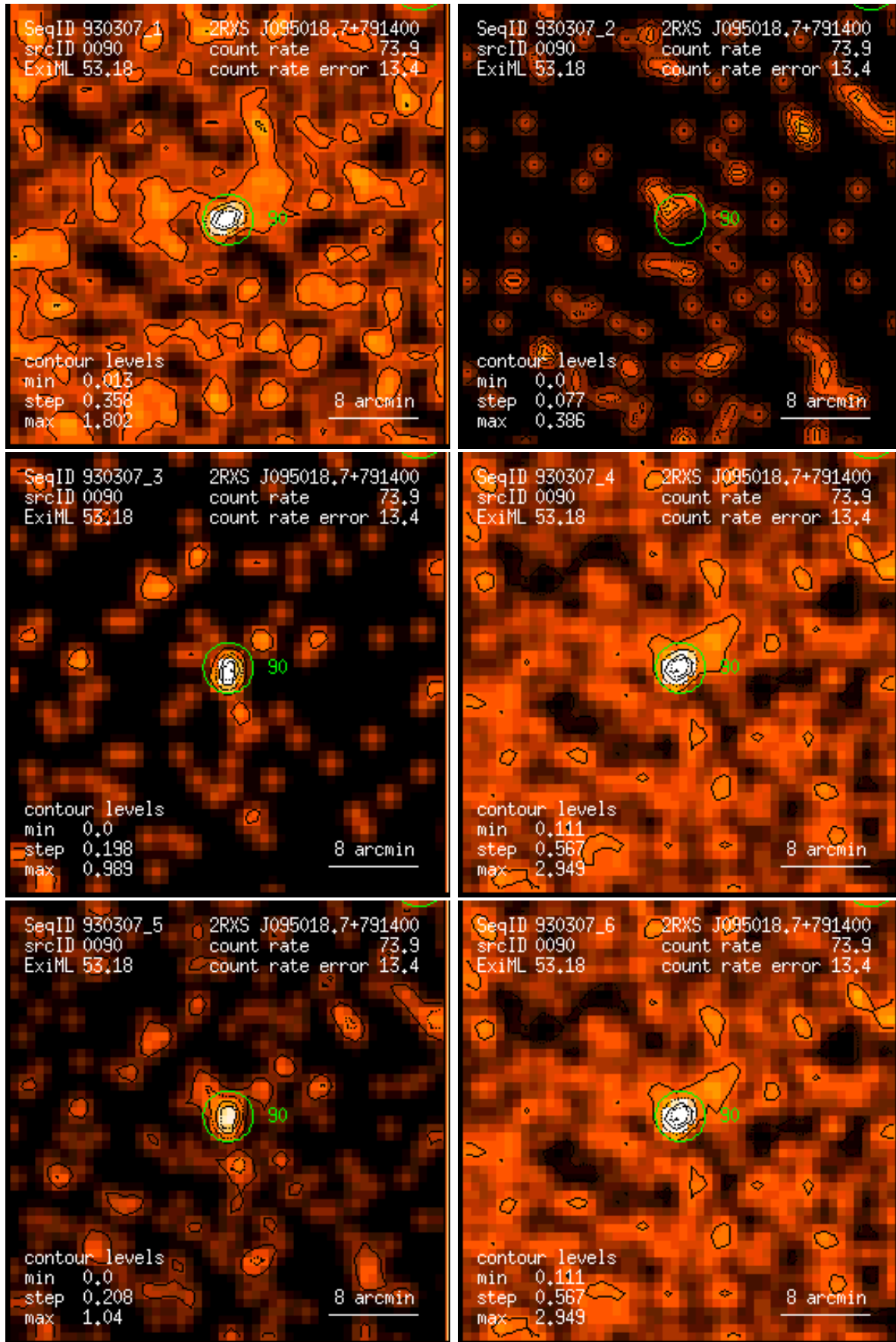
Figure 90: RASS 930307: detection 0090: band rate images, Gaussian filter: (1) PSPC channels 11 – 41, (2) 52 – 90, (3) 91 – 201, (4) 11 – 235, (5) 52 – 201, (6) 11 – 201. Broad band rates in counts/ks. Band rate contour levels in counts/ks/arcmin 2 .
