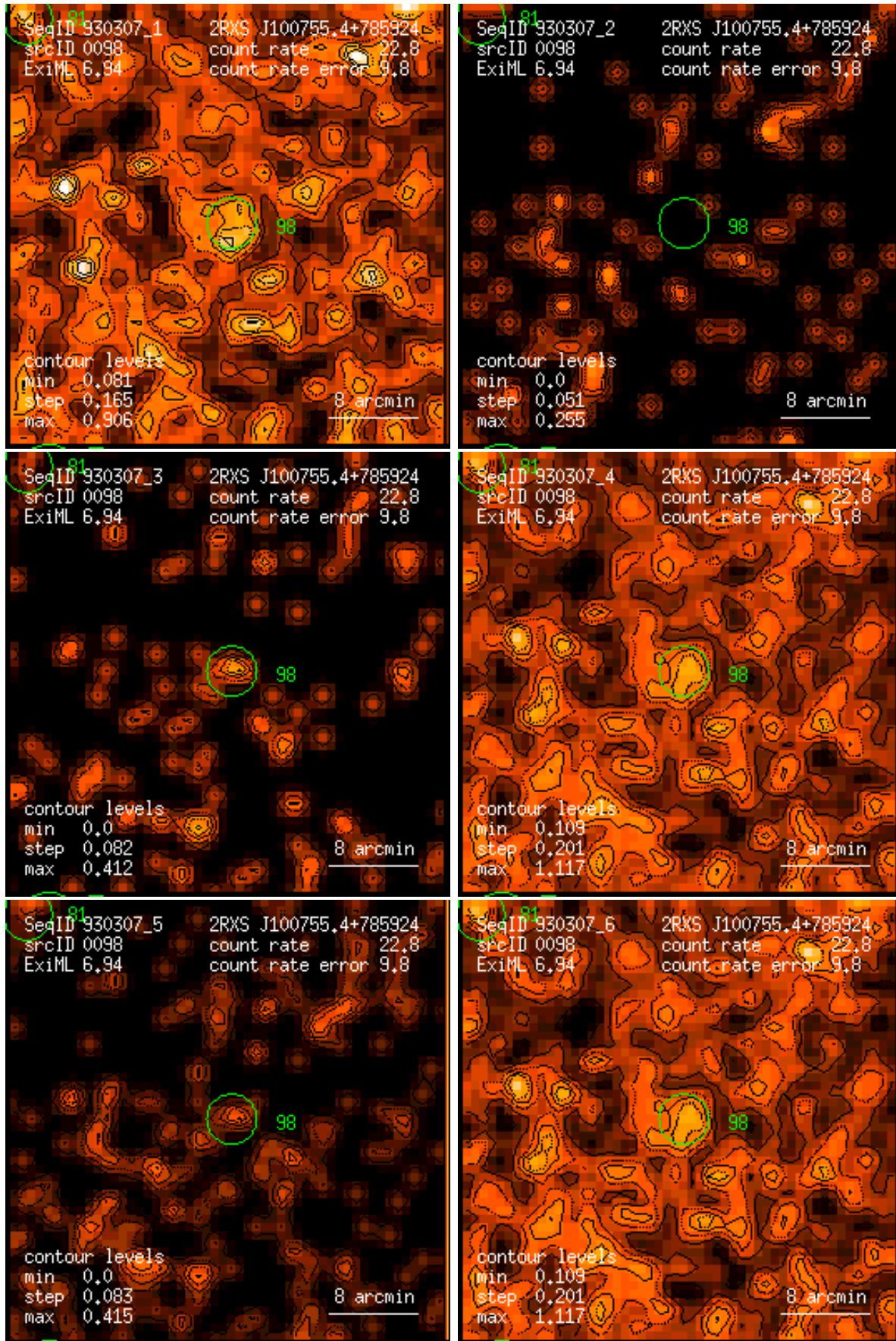
Figure 98: RASS 930307: detection 0098: band rate images, Gaussian filter: (1) PSPC channels 11 – 41, (2) 52 – 90, (3) 91 – 201, (4) 11 – 235, (5) 52 – 201, (6) 11 – 201. Broad band rates in counts/ks. Band rate contour levels in counts/ks/arcmin 2 .
