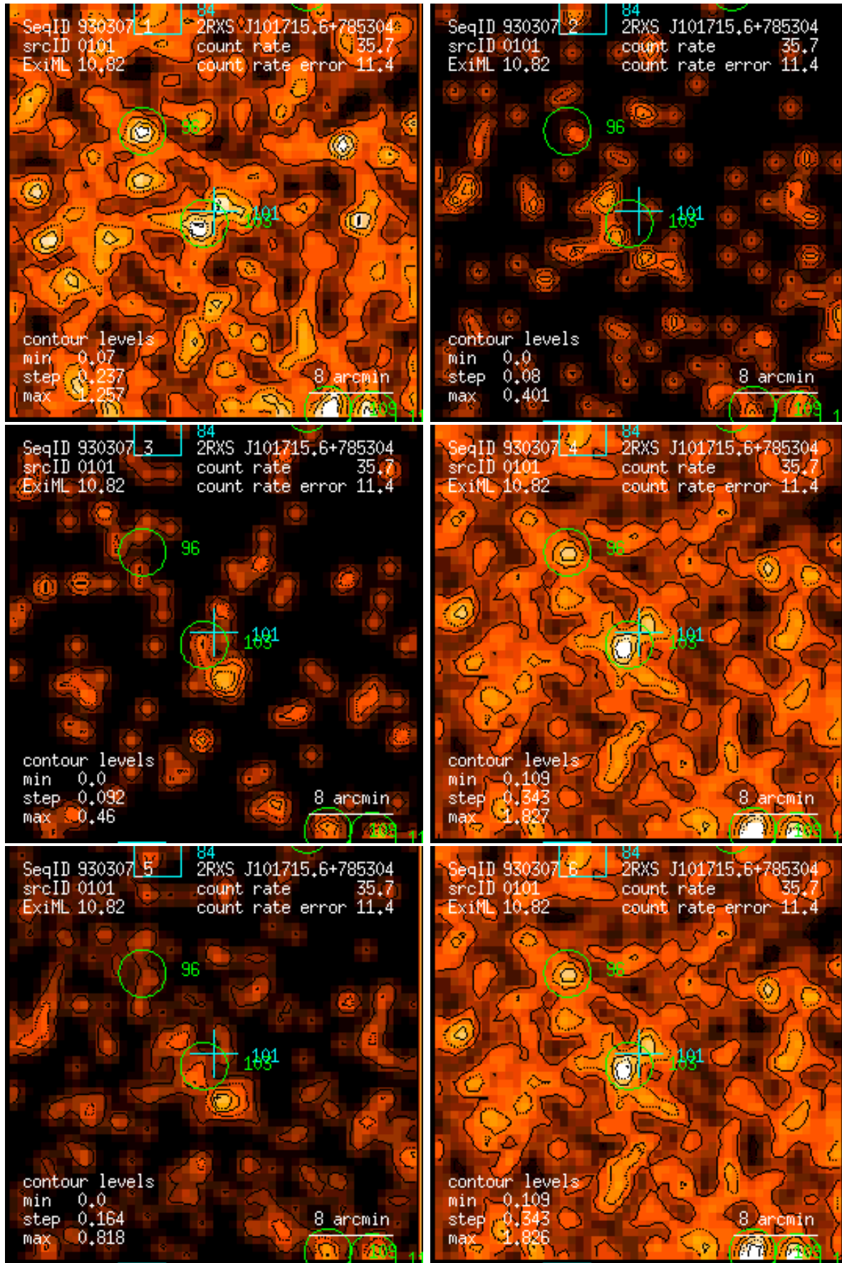
Figure 101: RASS 930307: detection 0101: band rate images, Gaussian filter: (1) PSPC channels 11 – 41, (2) 52 – 90, (3) 91 – 201, (4) 11 – 235, (5) 52 – 201, (6) 11 – 201. Broad band rates in counts/ks. Band rate contour levels in counts/ks/arcmin 2 .
