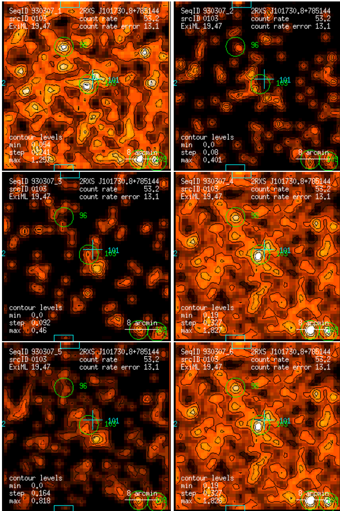
Figure 103: RASS 930307: detection 0103: band rate images, Gaussian filter: (1) PSPC channels 11 – 41, (2) 52 – 90, (3) 91 – 201, (4) 11 – 235, (5) 52 – 201, (6) 11 – 201. Broad band rates in counts/ks. Band rate contour levels in counts/ks/arcmin 2 .
