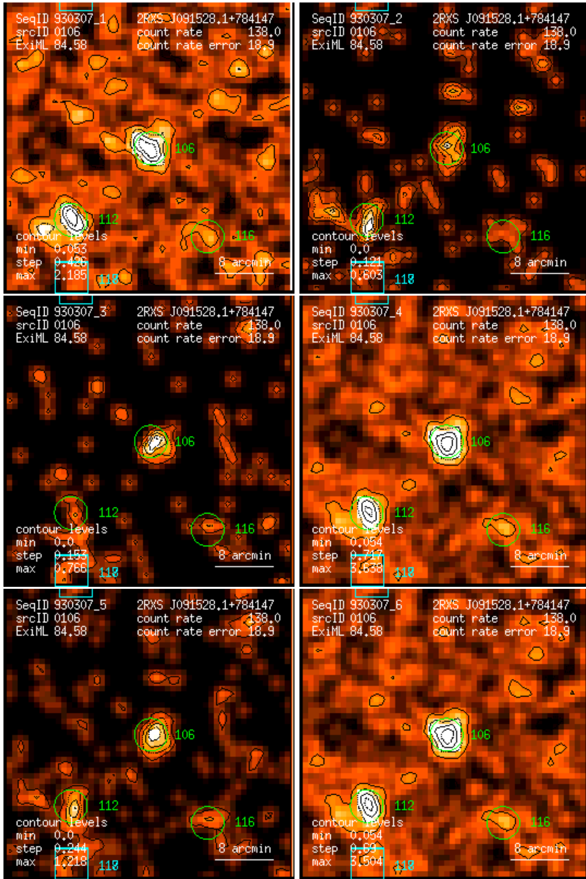
Figure 106: RASS 930307: detection 0106: band rate images, Gaussian filter: (1) PSPC channels 11 – 41, (2) 52 – 90, (3) 91 – 201, (4) 11 – 235, (5) 52 – 201, (6) 11 – 201. Broad band rates in counts/ks. Band rate contour levels in counts/ks/arcmin 2 .
