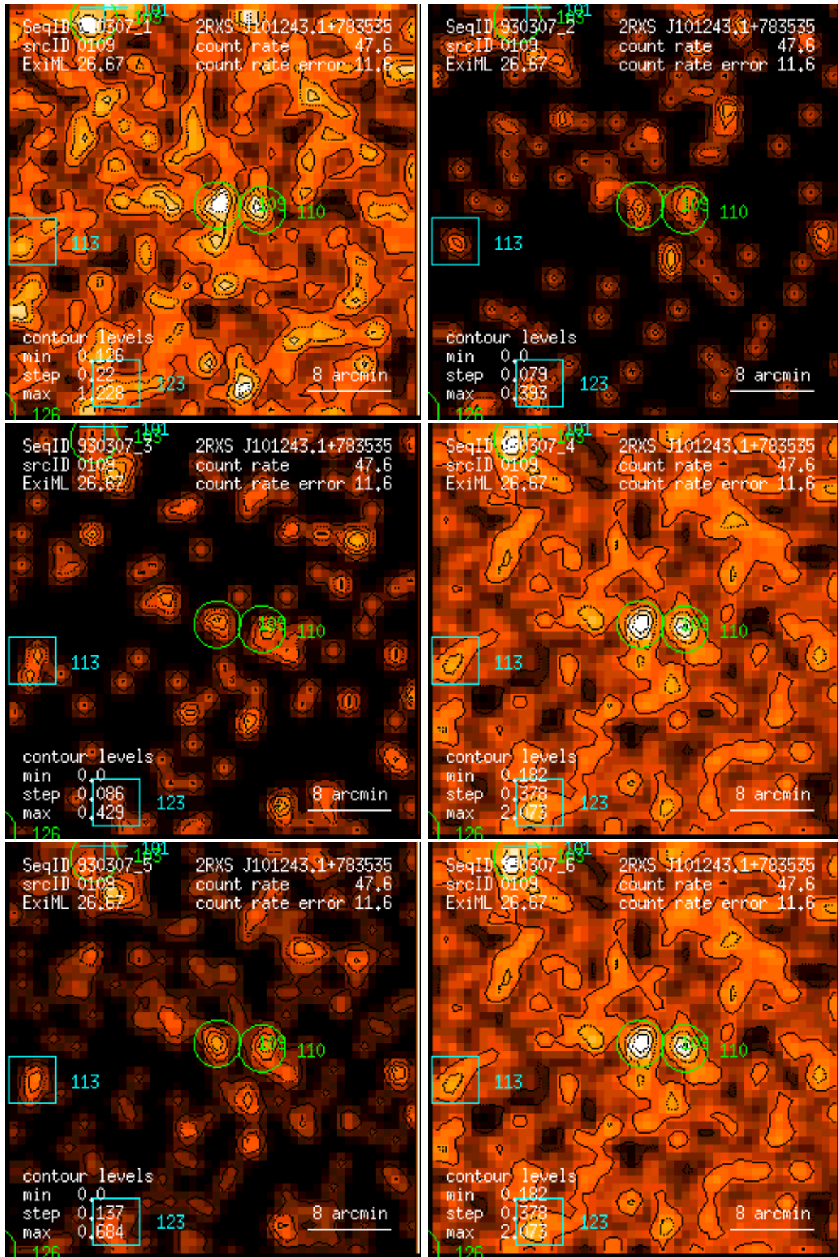
Figure 109: RASS 930307: detection 0109: band rate images, Gaussian filter: (1) PSPC channels 11 – 41, (2) 52 – 90, (3) 91 – 201, (4) 11 – 235, (5) 52 – 201, (6) 11 – 201. Broad band rates in counts/ks. Band rate contour levels in counts/ks/arcmin 2 .
