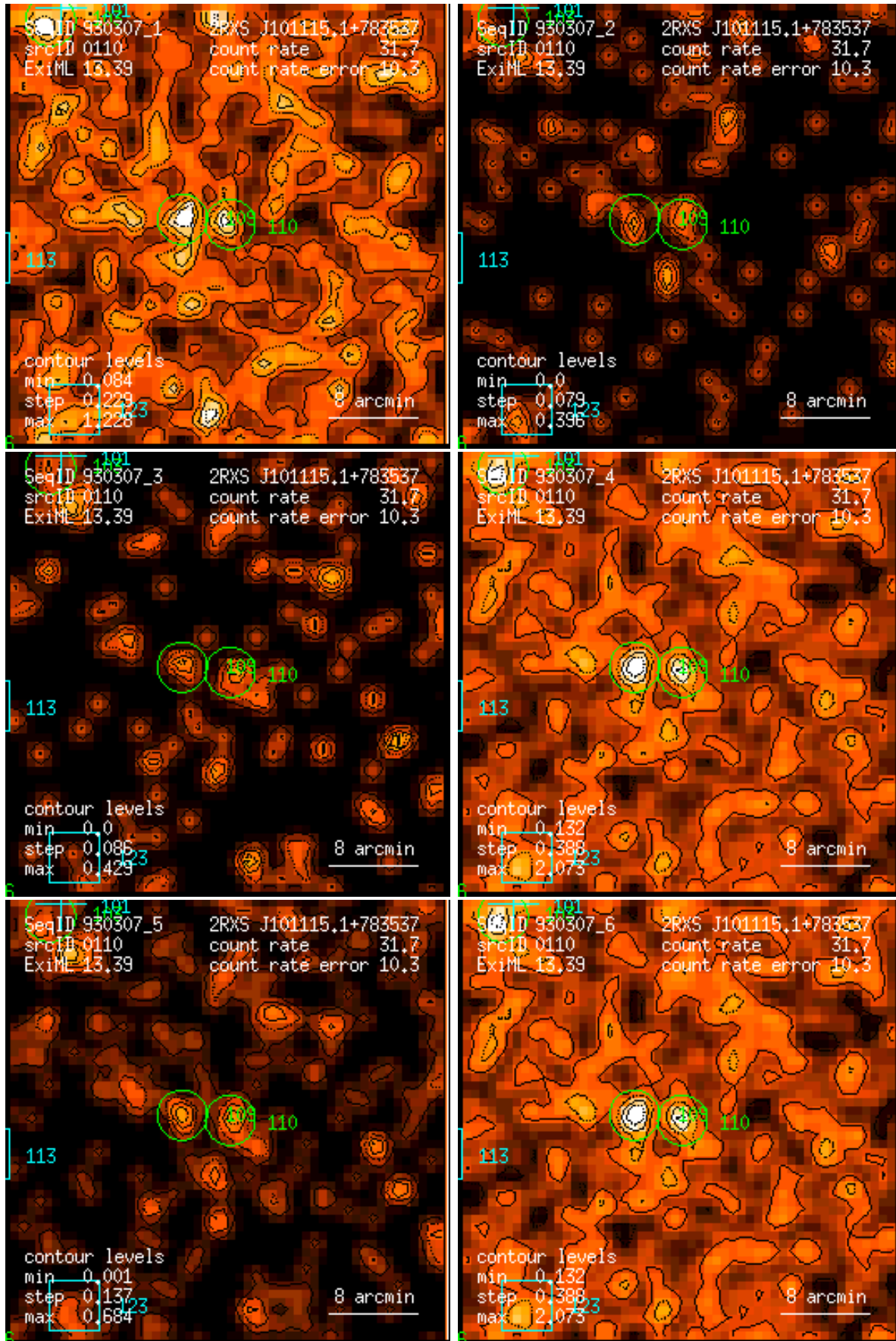
Figure 110: RASS 930307: detection 0110: band rate images, Gaussian filter: (1) PSPC channels 11 – 41, (2) 52 – 90, (3) 91 – 201, (4) 11 – 235, (5) 52 – 201, (6) 11 – 201. Broad band rates in counts/ks. Band rate contour levels in counts/ks/arcmin 2 .
