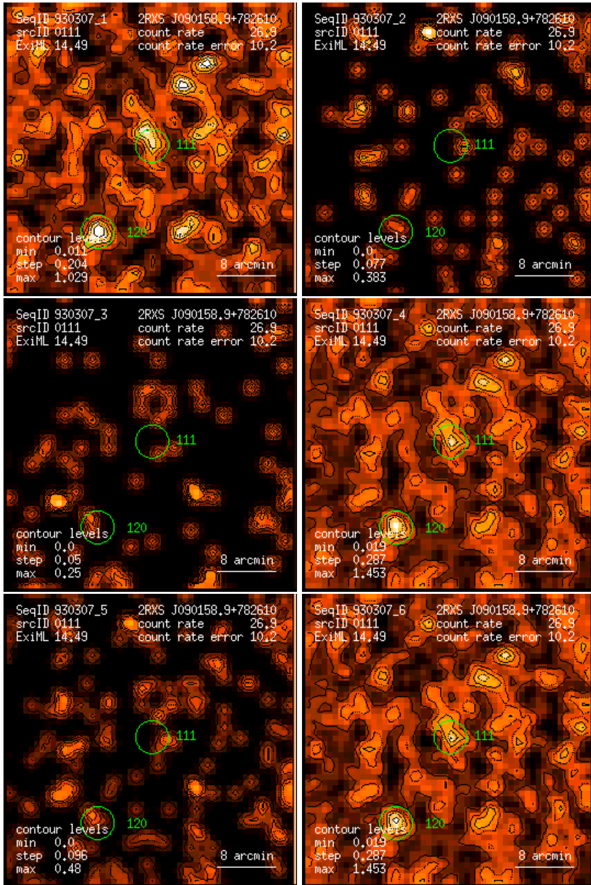
Figure 111: RASS 930307: detection 0111: band rate images, Gaussian filter: (1) PSPC channels 11 – 41, (2) 52 – 90, (3) 91 – 201, (4) 11 – 235, (5) 52 – 201, (6) 11 – 201. Broad band rates in counts/ks. Band rate contour levels in counts/ks/arcmin 2 .
