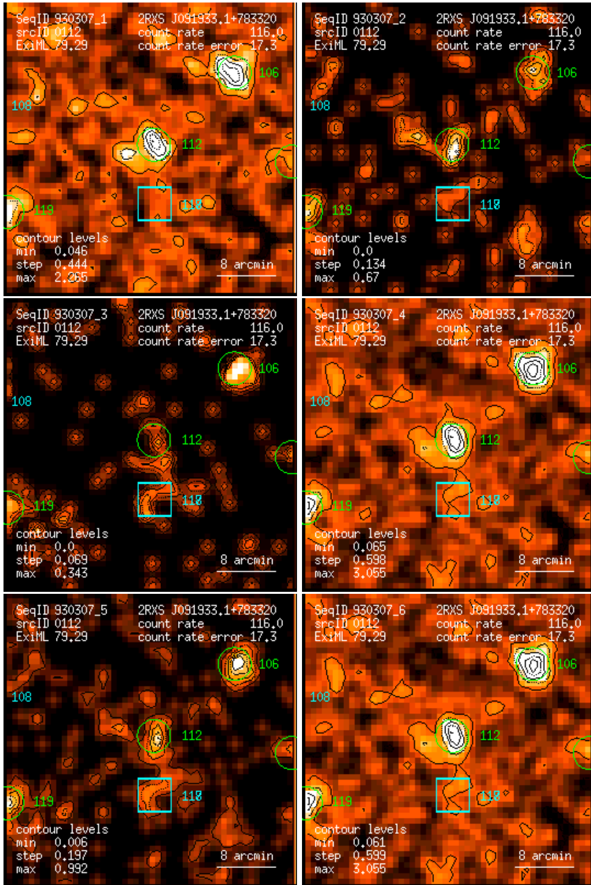
Figure 112: RASS 930307: detection 0112: band rate images, Gaussian filter: (1) PSPC channels 11 – 41, (2) 52 – 90, (3) 91 – 201, (4) 11 – 235, (5) 52 – 201, (6) 11 – 201. Broad band rates in counts/ks. Band rate contour levels in counts/ks/arcmin 2 .
