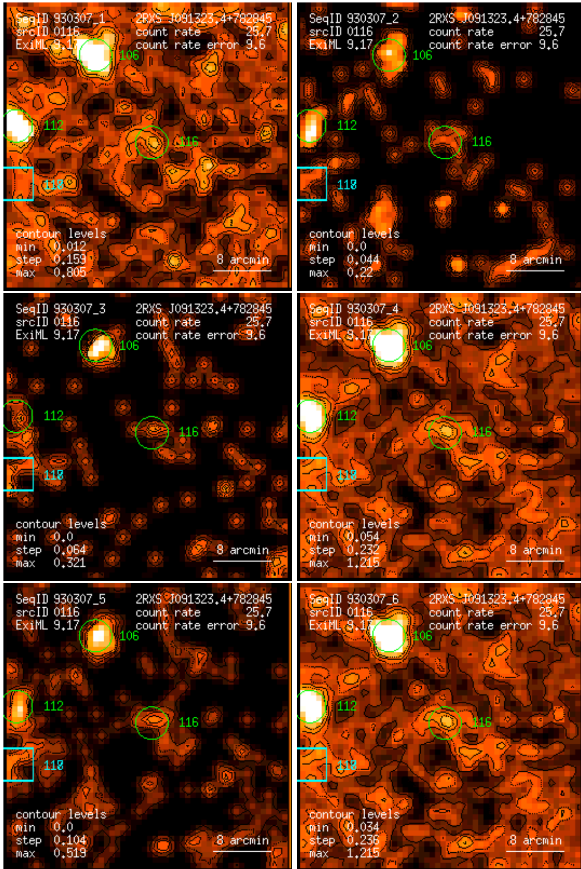
Figure 116: RASS 930307: detection 0116: band rate images, Gaussian filter: (1) PSPC channels 11 – 41, (2) 52 – 90, (3) 91 – 201, (4) 11 – 235, (5) 52 – 201, (6) 11 – 201. Broad band rates in counts/ks. Band rate contour levels in counts/ks/arcmin 2 .
