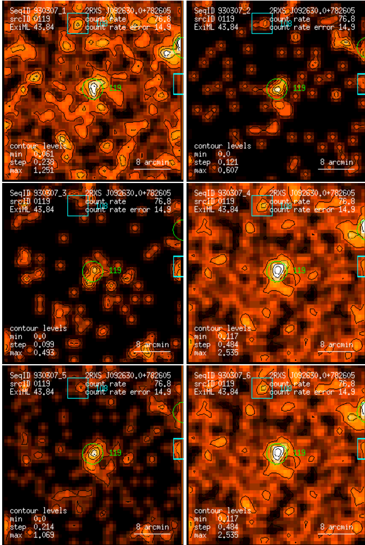
Figure 119: RASS 930307: detection 0119: band rate images, Gaussian filter: (1) PSPC channels 11 – 41, (2) 52 – 90, (3) 91 – 201, (4) 11 – 235, (5) 52 – 201, (6) 11 – 201. Broad band rates in counts/ks. Band rate contour levels in counts/ks/arcmin 2 .
