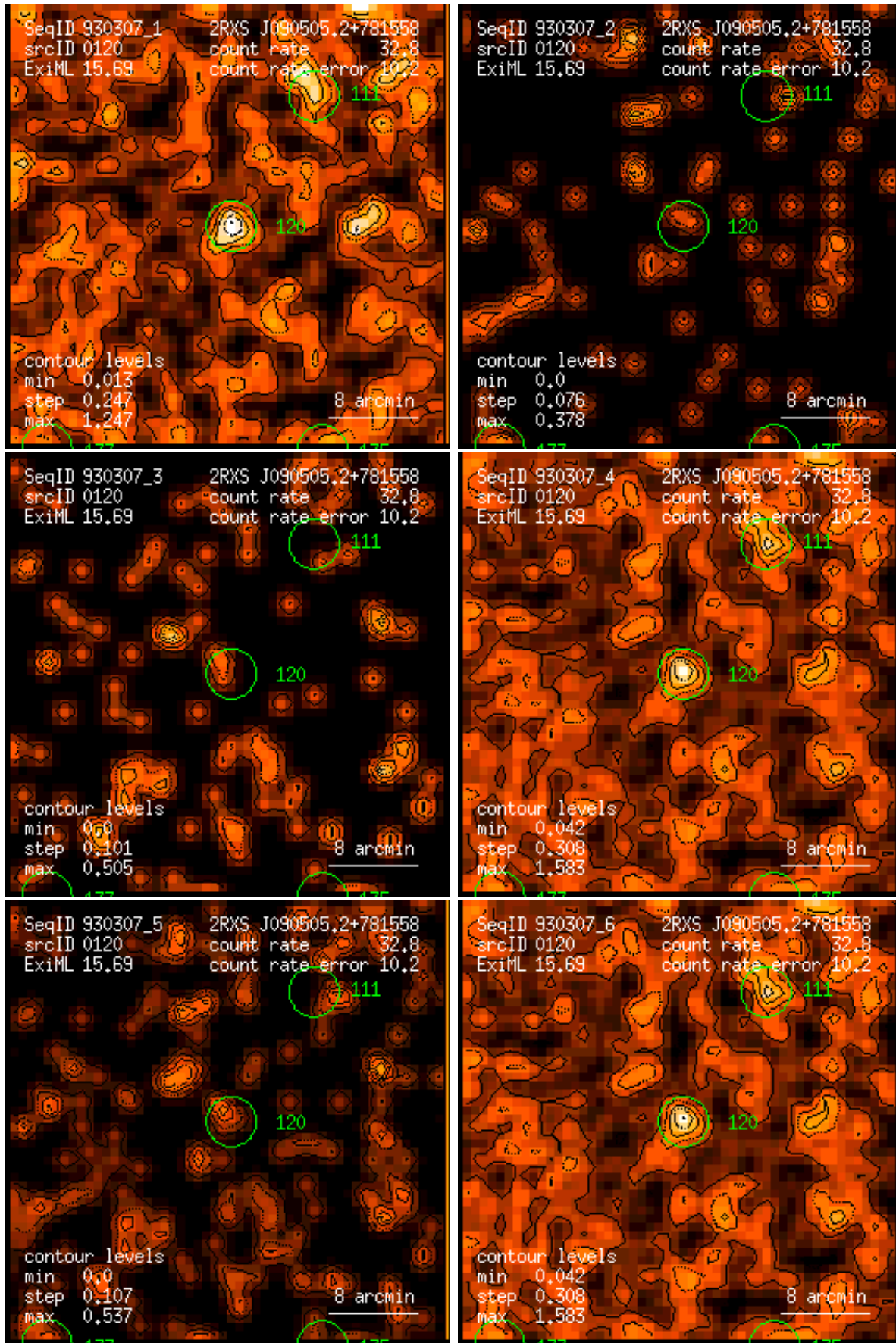
Figure 120: RASS 930307: detection 0120: band rate images, Gaussian filter: (1) PSPC channels 11 – 41, (2) 52 – 90, (3) 91 – 201, (4) 11 – 235, (5) 52 – 201, (6) 11 – 201. Broad band rates in counts/ks. Band rate contour levels in counts/ks/arcmin 2 .
