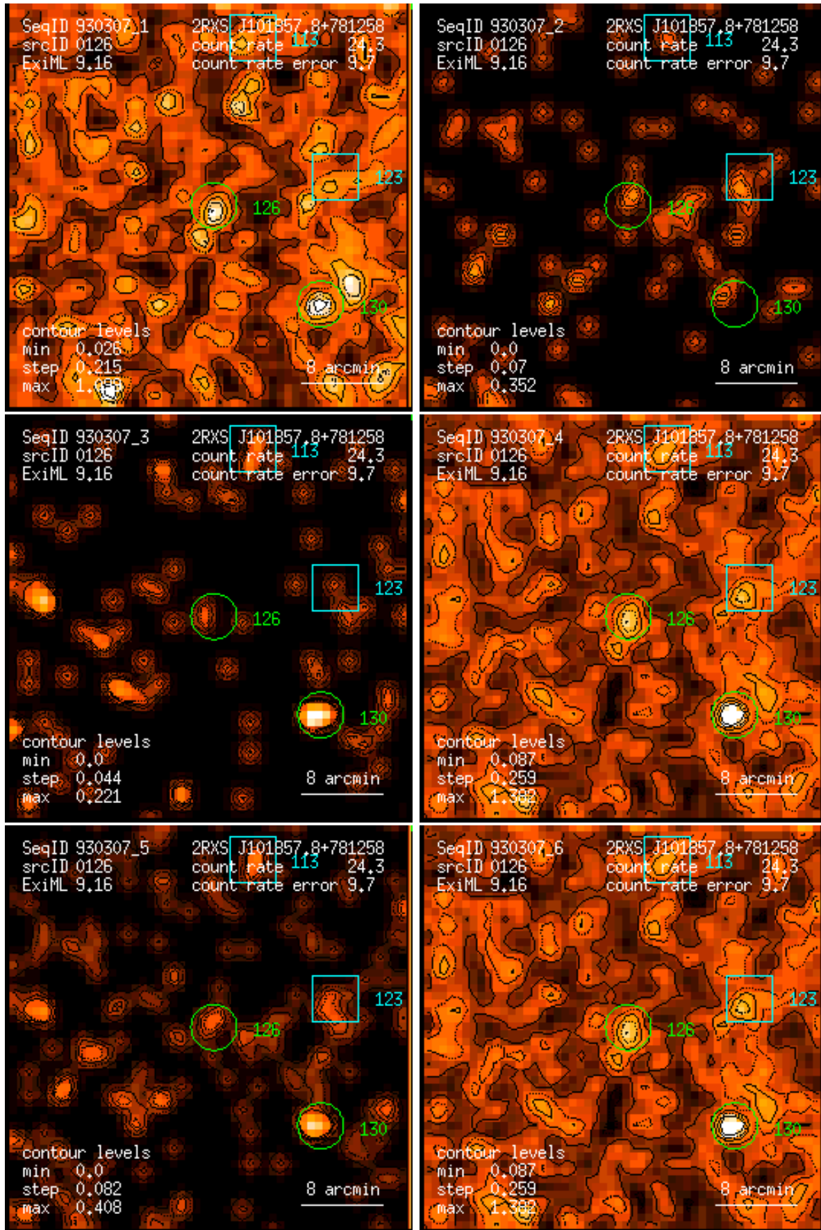
Figure 126: RASS 930307: detection 0126: band rate images, Gaussian filter: (1) PSPC channels 11 – 41, (2) 52 – 90, (3) 91 – 201, (4) 11 – 235, (5) 52 – 201, (6) 11 – 201. Broad band rates in counts/ks. Band rate contour levels in counts/ks/arcmin 2 .
