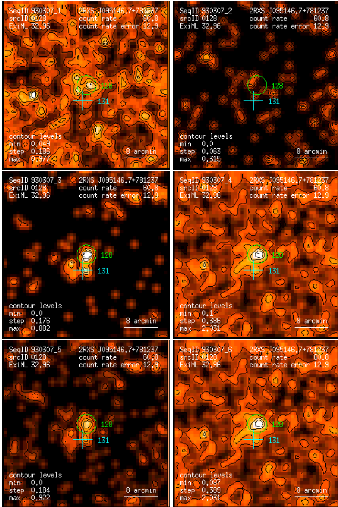
Figure 128: RASS 930307: detection 0128: band rate images, Gaussian filter: (1) PSPC channels 11 – 41, (2) 52 – 90, (3) 91 – 201, (4) 11 – 235, (5) 52 – 201, (6) 11 – 201. Broad band rates in counts/ks. Band rate contour levels in counts/ks/arcmin 2 .
