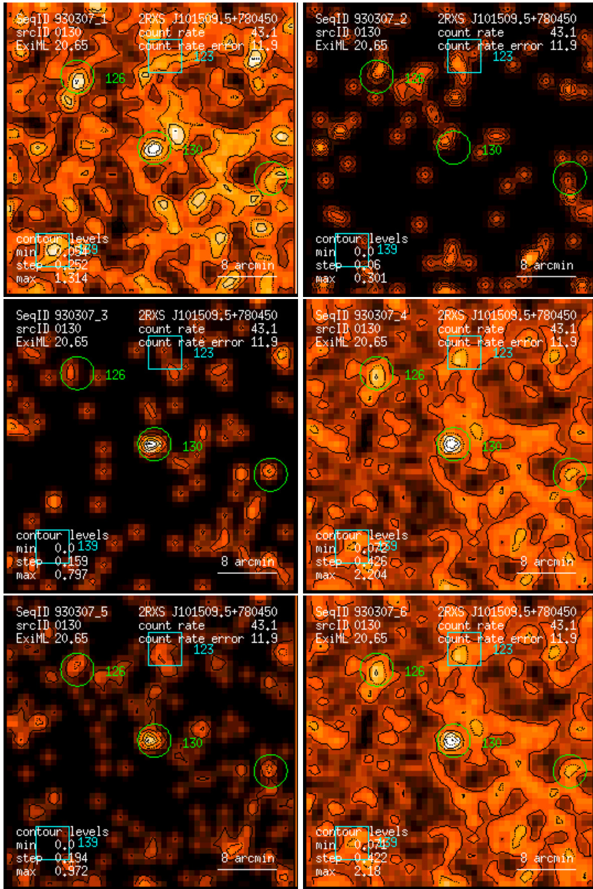
Figure 130: RASS 930307: detection 0130: band rate images, Gaussian filter: (1) PSPC channels 11 – 41, (2) 52 – 90, (3) 91 – 201, (4) 11 – 235, (5) 52 – 201, (6) 11 – 201. Broad band rates in counts/ks. Band rate contour levels in counts/ks/arcmin 2 .
