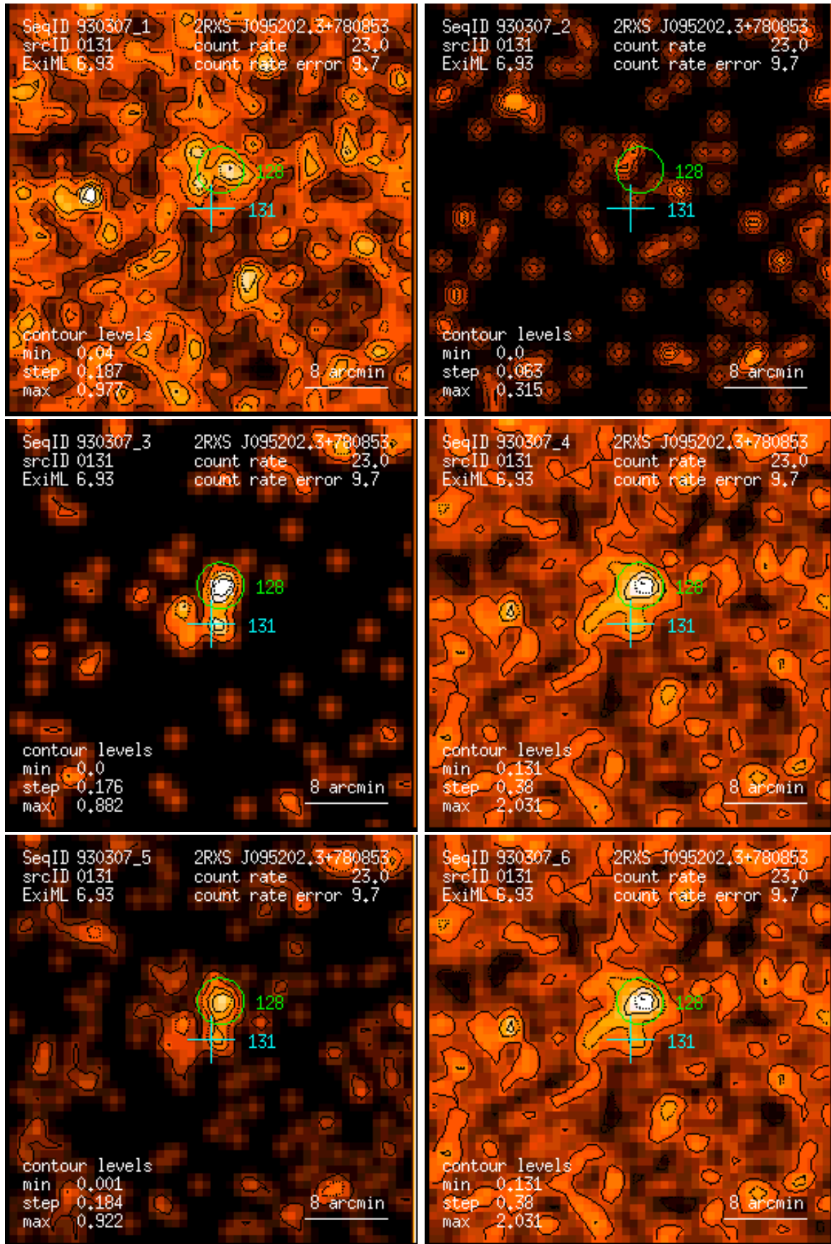
Figure 131: RASS 930307: detection 0131: band rate images, Gaussian filter: (1) PSPC channels 11 – 41, (2) 52 – 90, (3) 91 – 201, (4) 11 – 235, (5) 52 – 201, (6) 11 – 201. Broad band rates in counts/ks. Band rate contour levels in counts/ks/arcmin 2 .
