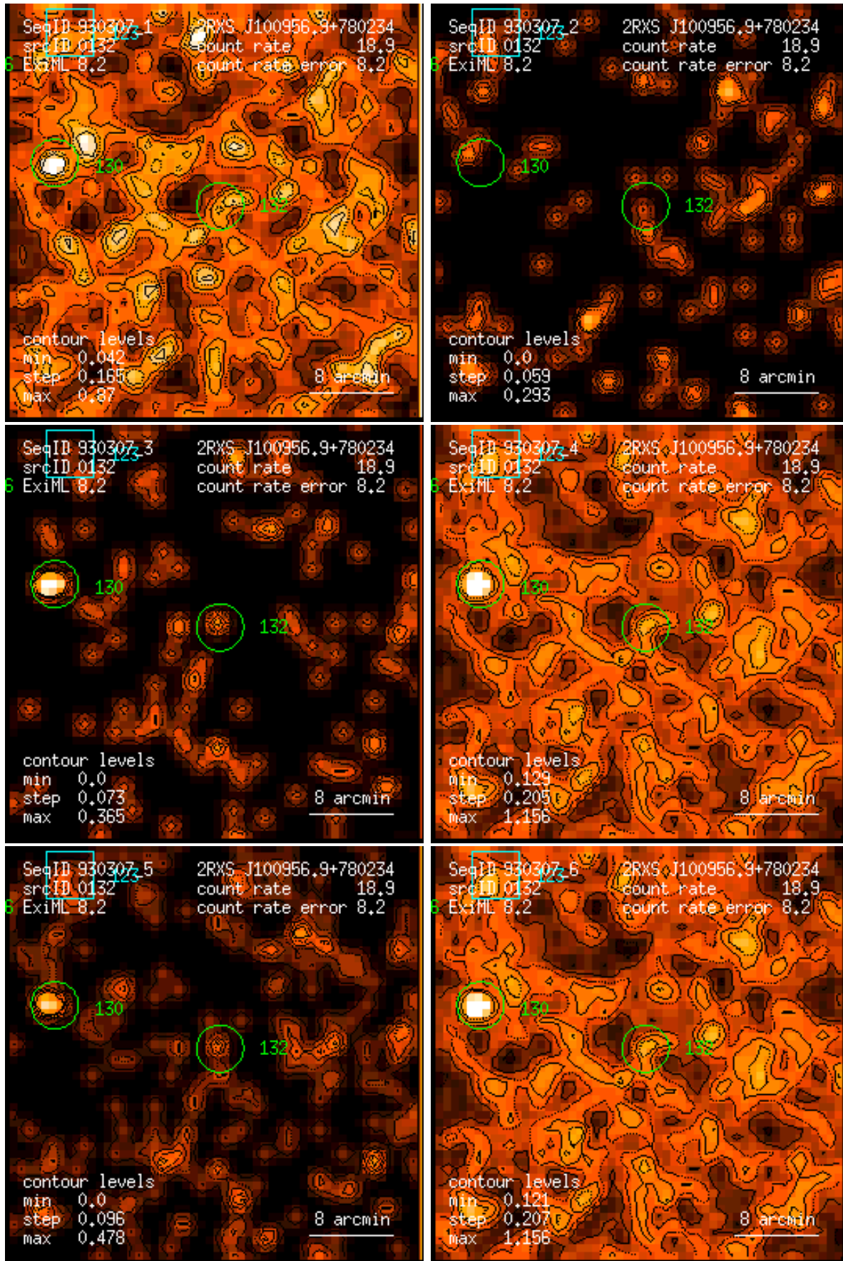
Figure 132: RASS 930307: detection 0132: band rate images, Gaussian filter: (1) PSPC channels 11 – 41, (2) 52 – 90, (3) 91 – 201, (4) 11 – 235, (5) 52 – 201, (6) 11 – 201. Broad band rates in counts/ks. Band rate contour levels in counts/ks/arcmin 2 .
