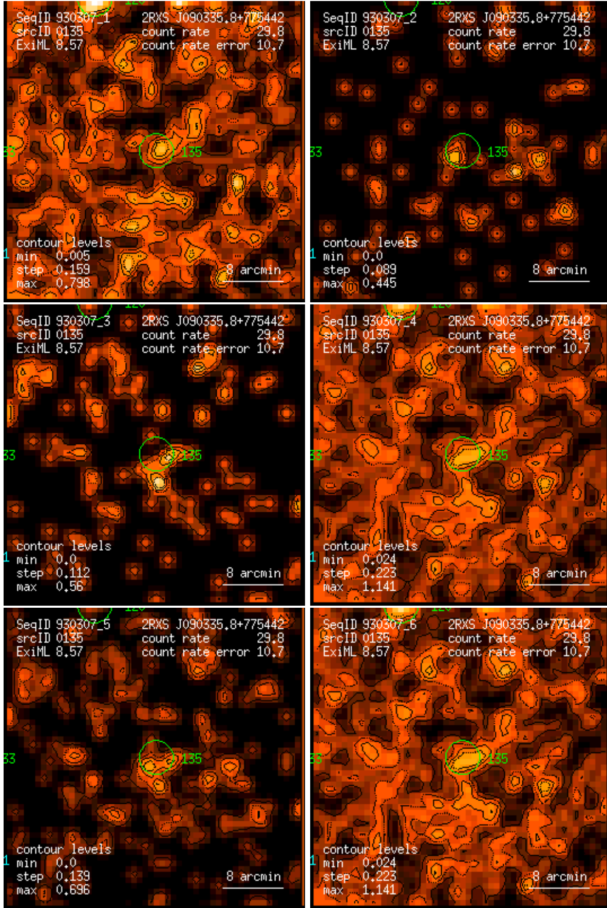
Figure 135: RASS 930307: detection 0135: band rate images, Gaussian filter: (1) PSPC channels 11 – 41, (2) 52 – 90, (3) 91 – 201, (4) 11 – 235, (5) 52 – 201, (6) 11 – 201. Broad band rates in counts/ks. Band rate contour levels in counts/ks/arcmin 2 .
