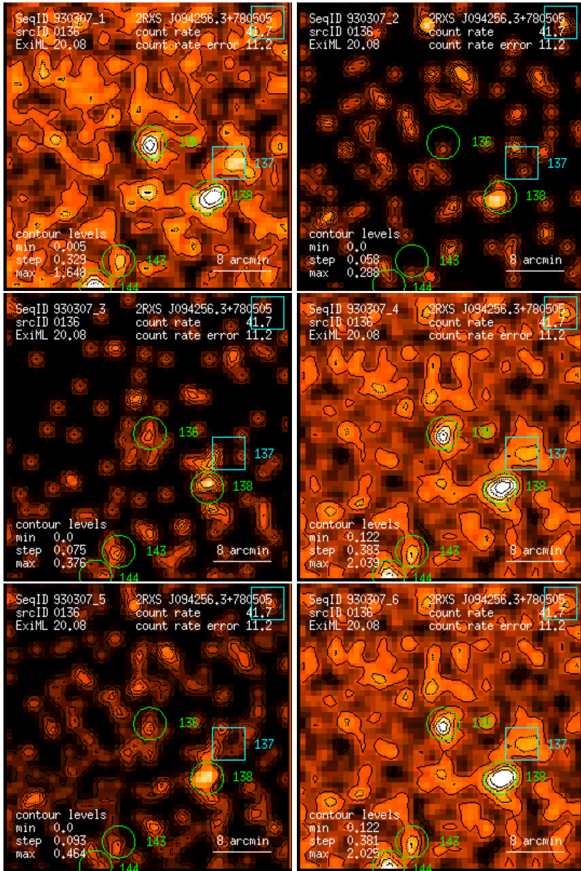
Figure 136: RASS 930307: detection 0136: band rate images, Gaussian filter: (1) PSPC channels 11 – 41, (2) 52 – 90, (3) 91 – 201, (4) 11 – 235, (5) 52 – 201, (6) 11 – 201. Broad band rates in counts/ks. Band rate contour levels in counts/ks/arcmin 2 .
