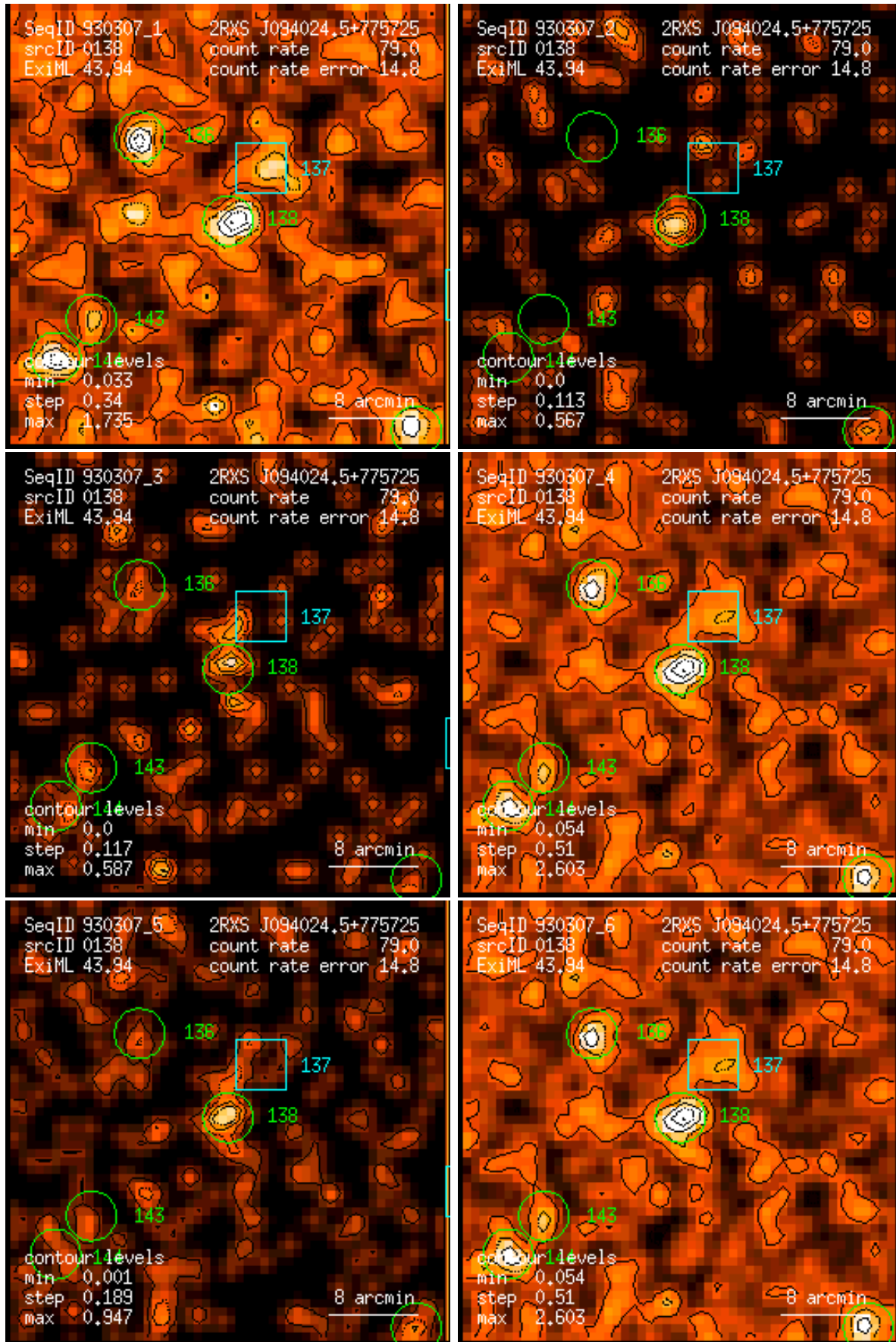
Figure 138: RASS 930307: detection 0138: band rate images, Gaussian filter: (1) PSPC channels 11 – 41, (2) 52 – 90, (3) 91 – 201, (4) 11 – 235, (5) 52 – 201, (6) 11 – 201. Broad band rates in counts/ks. Band rate contour levels in counts/ks/arcmin 2 .
