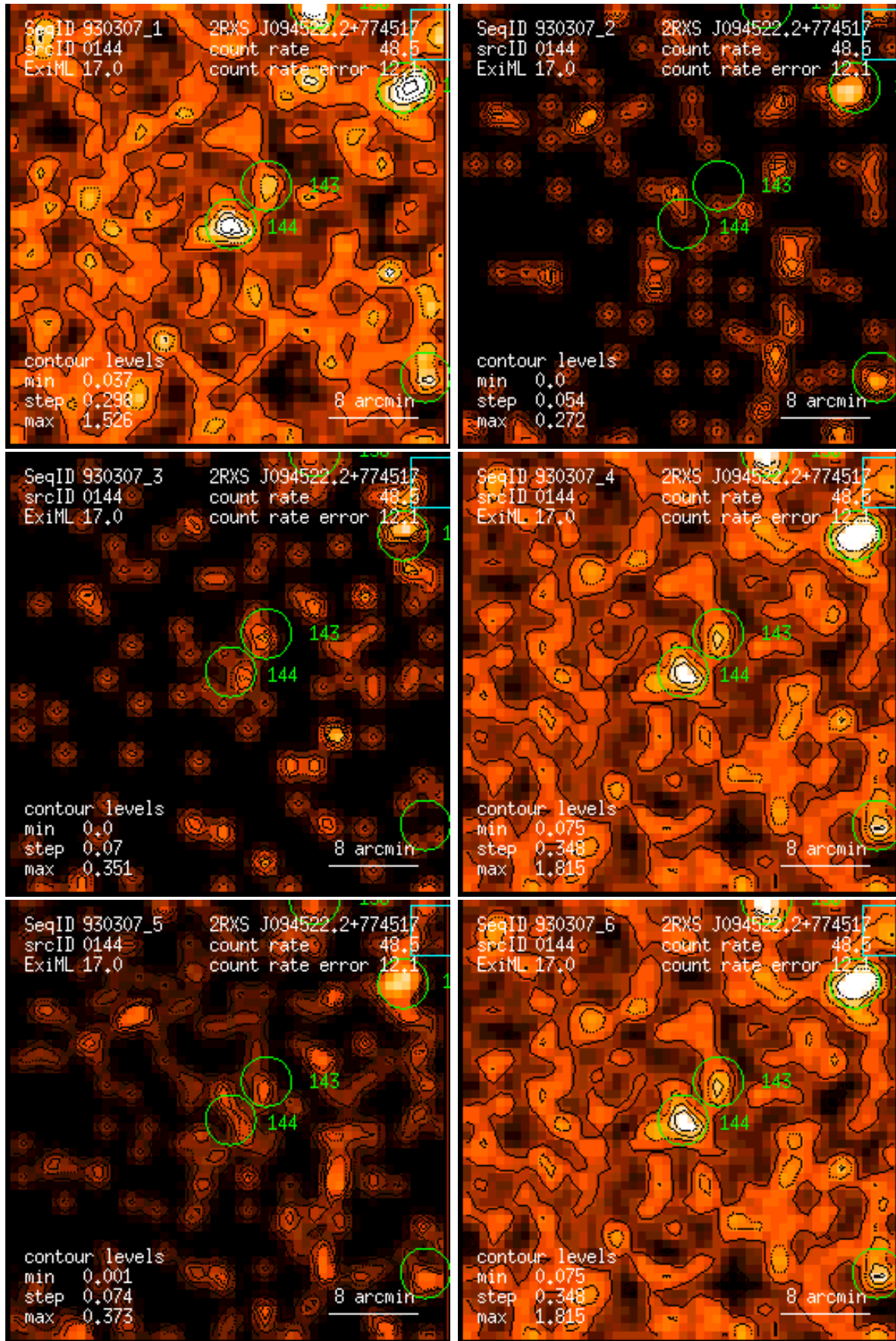
Figure 144: RASS 930307: detection 0144: band rate images, Gaussian filter: (1) PSPC channels 11 – 41, (2) 52 – 90, (3) 91 – 201, (4) 11 – 235, (5) 52 – 201, (6) 11 – 201. Broad band rates in counts/ks. Band rate contour levels in counts/ks/arcmin 2 .
