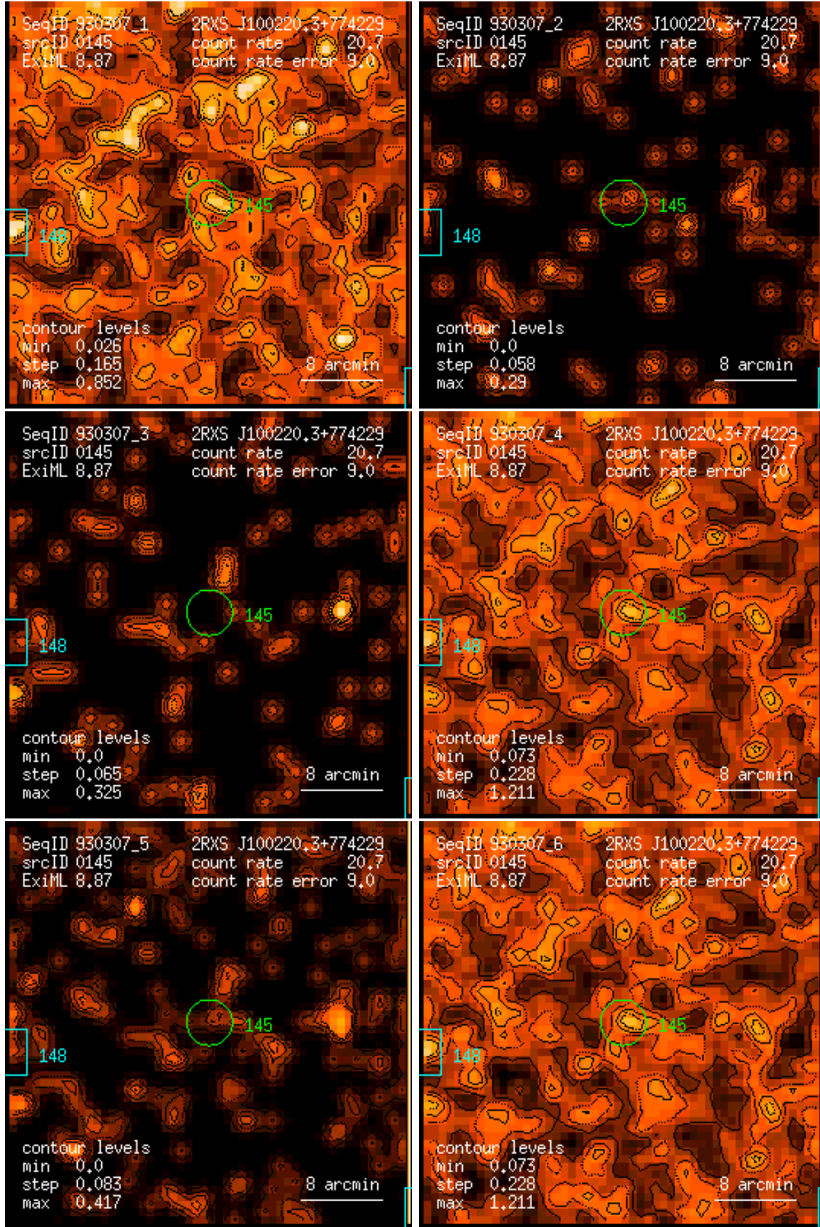
Figure 145: RASS 930307: detection 0145: band rate images, Gaussian filter: (1) PSPC channels 11 – 41, (2) 52 – 90, (3) 91 – 201, (4) 11 – 235, (5) 52 – 201, (6) 11 – 201. Broad band rates in counts/ks. Band rate contour levels in counts/ks/arcmin 2 .
