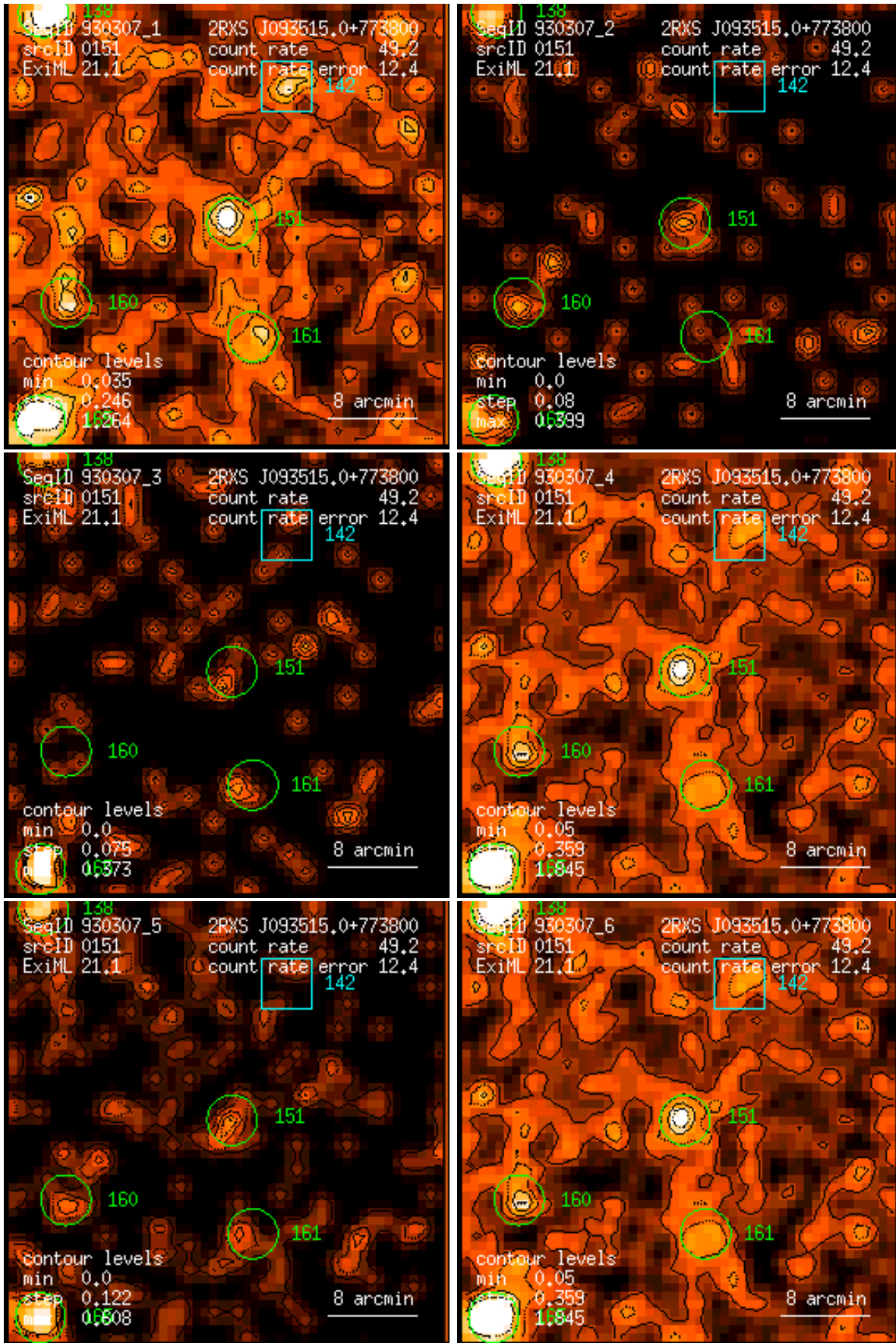
Figure 151: RASS 930307: detection 0151: band rate images, Gaussian filter: (1) PSPC channels 11 – 41, (2) 52 – 90, (3) 91 – 201, (4) 11 – 235, (5) 52 – 201, (6) 11 – 201. Broad band rates in counts/ks. Band rate contour levels in counts/ks/arcmin 2 .
