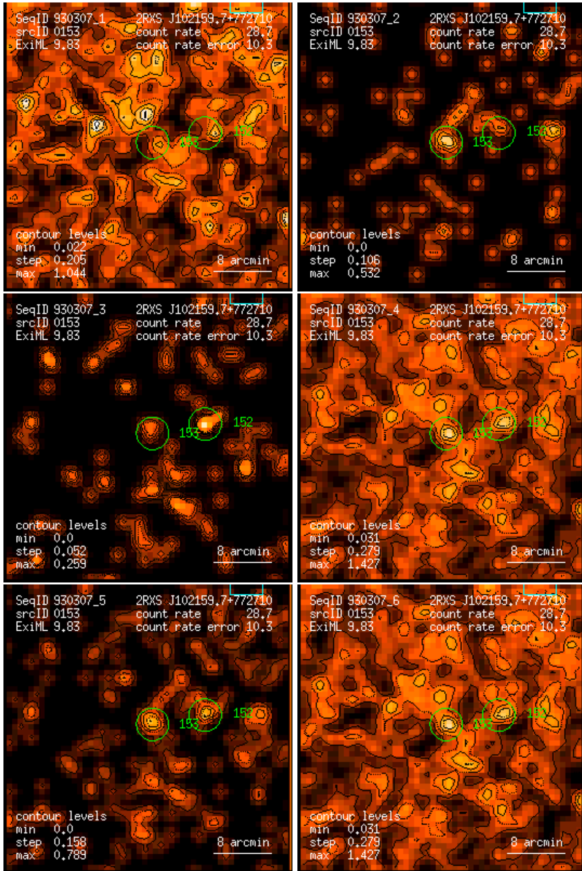
Figure 153: RASS 930307: detection 0153: band rate images, Gaussian filter: (1) PSPC channels 11 – 41, (2) 52 – 90, (3) 91 – 201, (4) 11 – 235, (5) 52 – 201, (6) 11 – 201. Broad band rates in counts/ks. Band rate contour levels in counts/ks/arcmin 2 .
