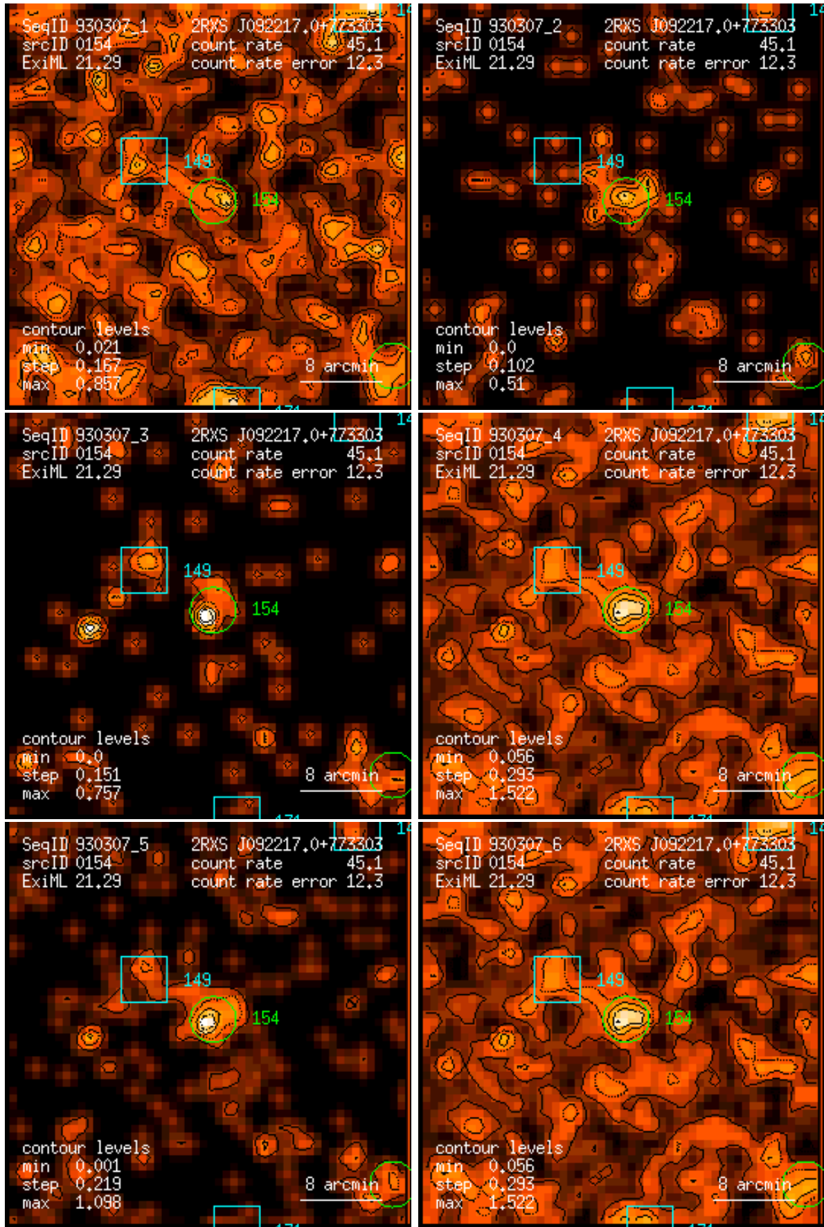
Figure 154: RASS 930307: detection 0154: band rate images, Gaussian filter: (1) PSPC channels 11 – 41, (2) 52 – 90, (3) 91 – 201, (4) 11 – 235, (5) 52 – 201, (6) 11 – 201. Broad band rates in counts/ks. Band rate contour levels in counts/ks/arcmin 2 .
