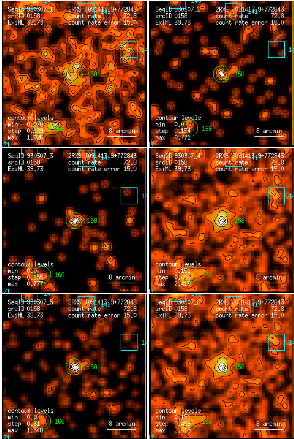
Figure 158: RASS 930307: detection 0158: band rate images, Gaussian filter: (1) PSPC channels 11 – 41, (2) 52 – 90, (3) 91 – 201, (4) 11 – 235, (5) 52 – 201, (6) 11 – 201. Broad band rates in counts/ks. Band rate contour levels in counts/ks/arcmin 2 .
