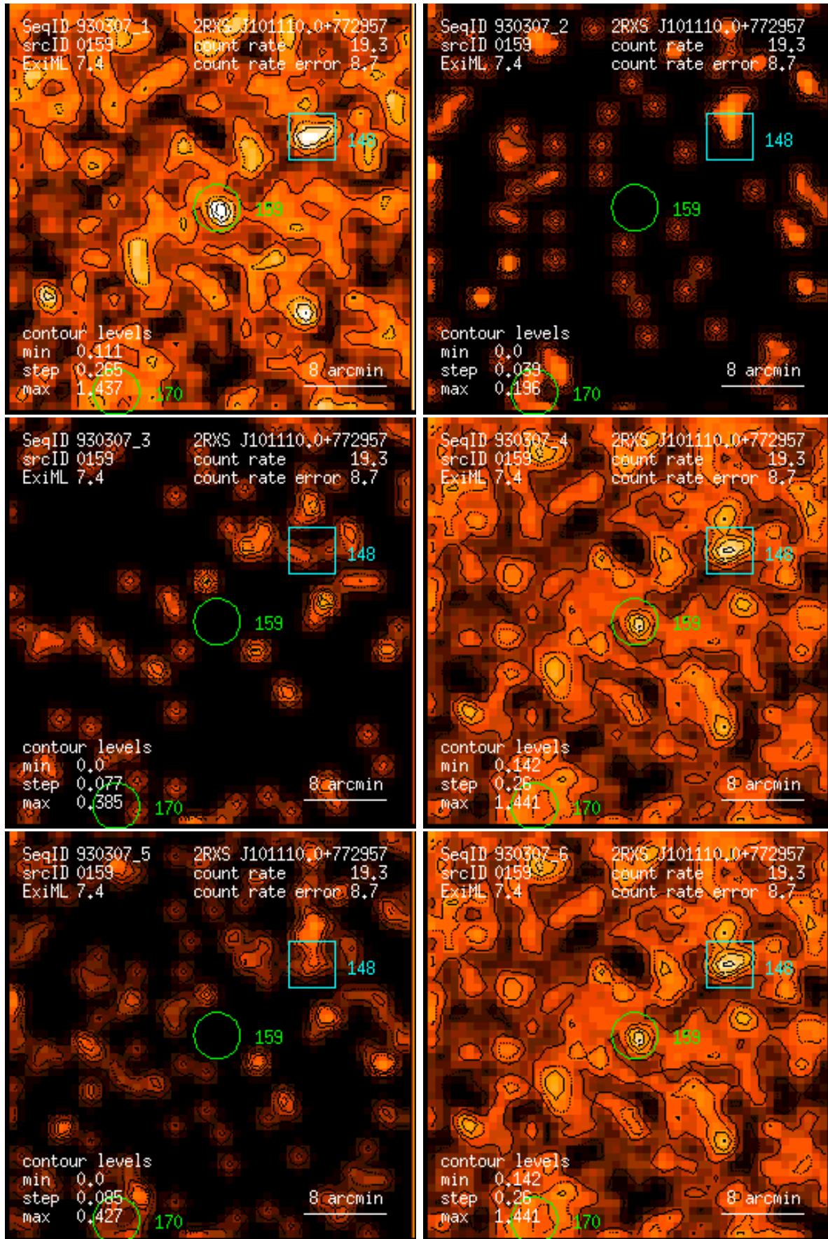
Figure 159: RASS 930307: detection 0159: band rate images, Gaussian filter: (1) PSPC channels 11 – 41, (2) 52 – 90, (3) 91 – 201, (4) 11 – 235, (5) 52 – 201, (6) 11 – 201. Broad band rates in counts/ks. Band rate contour levels in counts/ks/arcmin 2 .
