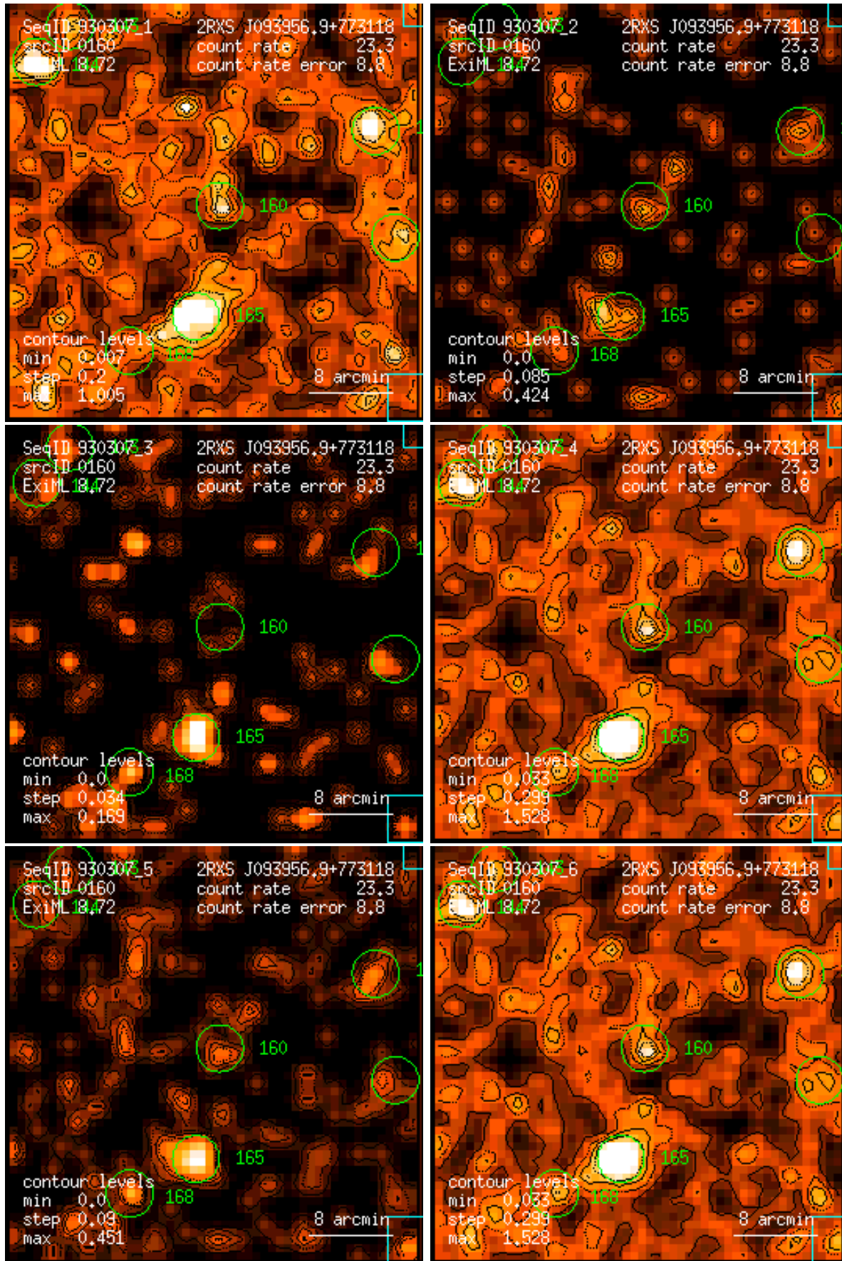
Figure 160: RASS 930307: detection 0160: band rate images, Gaussian filter: (1) PSPC channels 11 – 41, (2) 52 – 90, (3) 91 – 201, (4) 11 – 235, (5) 52 – 201, (6) 11 – 201. Broad band rates in counts/ks. Band rate contour levels in counts/ks/arcmin 2 .
