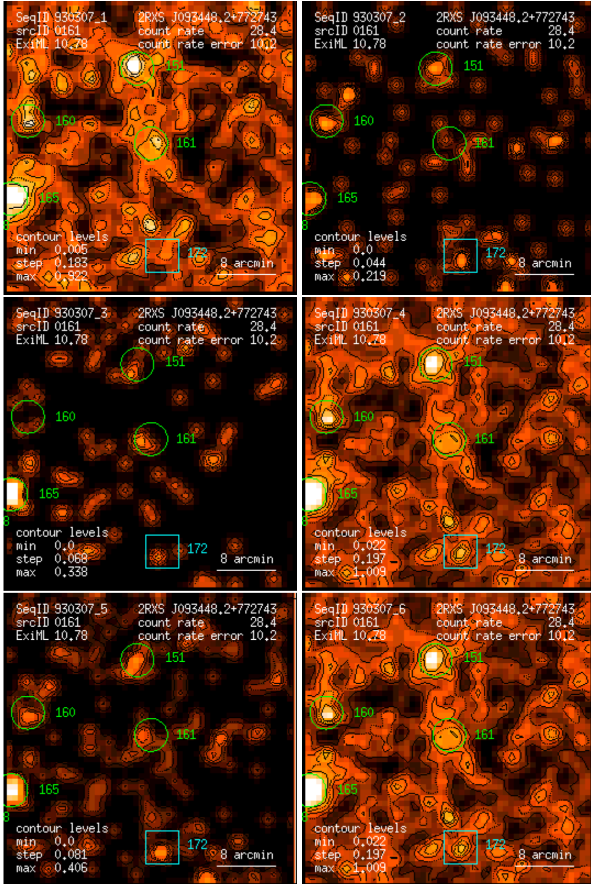
Figure 161: RASS 930307: detection 0161: band rate images, Gaussian filter: (1) PSPC channels 11 – 41, (2) 52 – 90, (3) 91 – 201, (4) 11 – 235, (5) 52 – 201, (6) 11 – 201. Broad band rates in counts/ks. Band rate contour levels in counts/ks/arcmin 2 .
